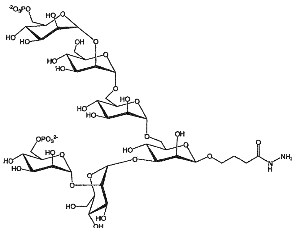
Formula 1a
