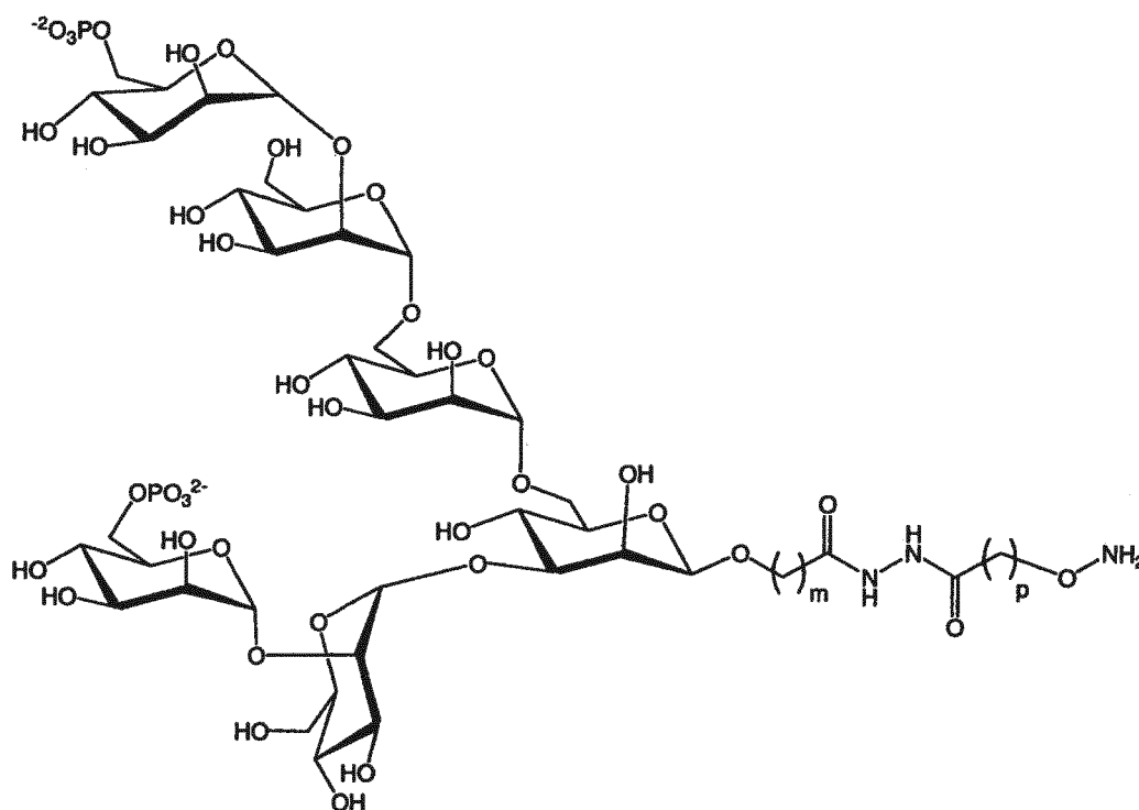
Formula IV
