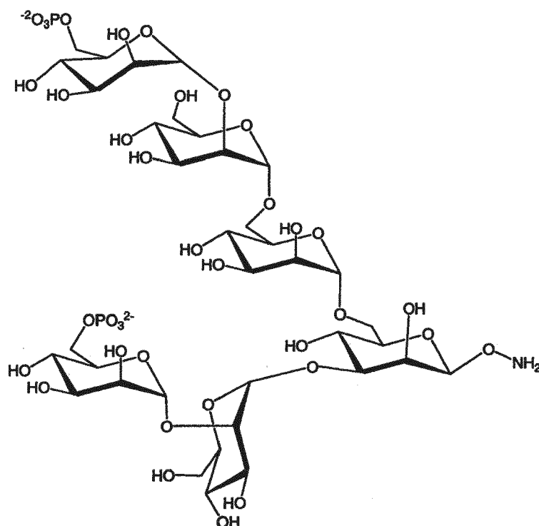
Formula V
