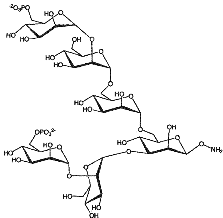
Formula V
