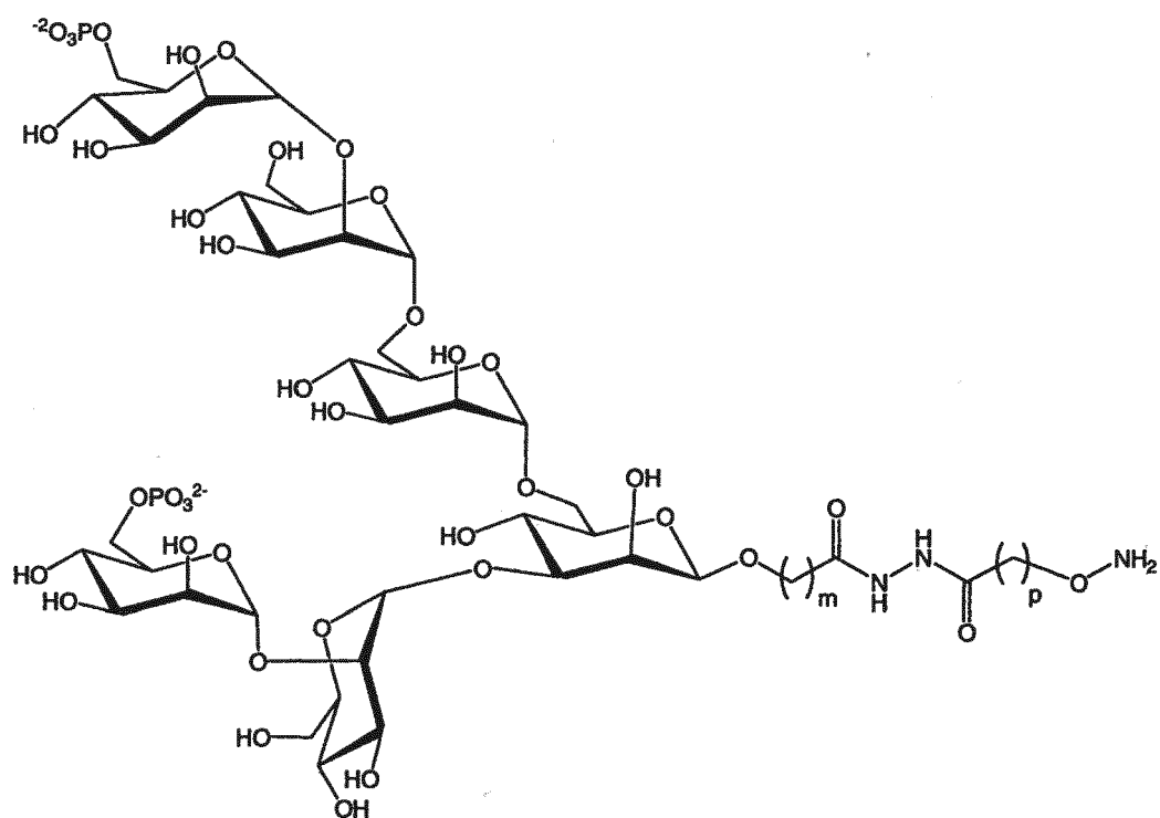
Formula IV
