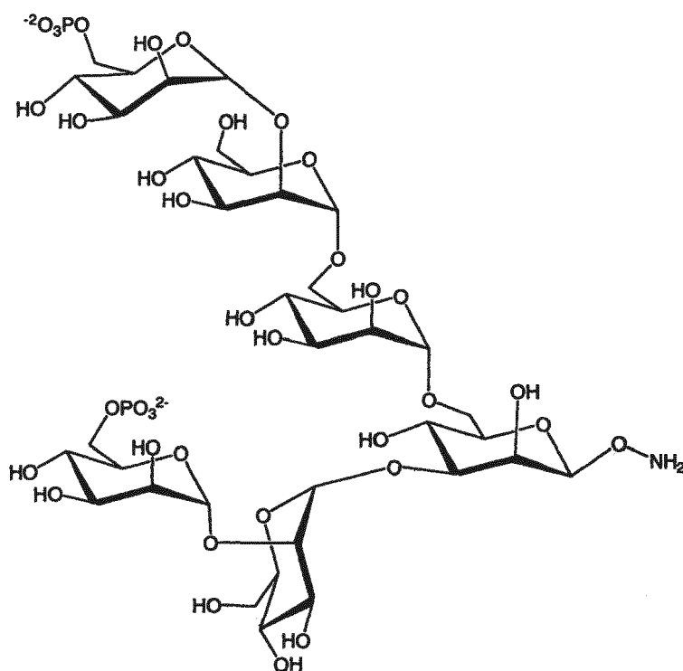
Formula V
