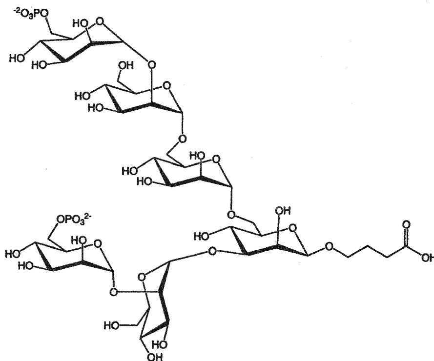
Formula Ib
