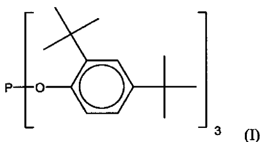
Tris(2,4-di-t-butylphenyl)phosphite
