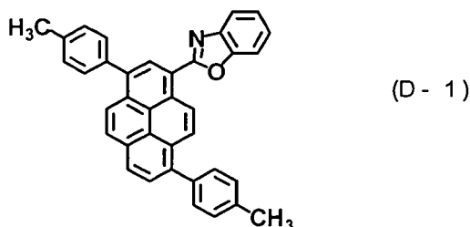
[Chemical Formula 54]
