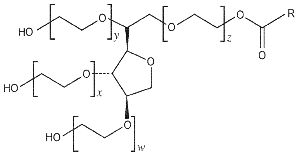
Polyoxyethylene sorbitan monoester
