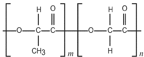
Poly(lactide-co-glycolide)
