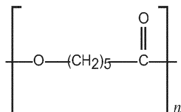
Polycaprolactone
