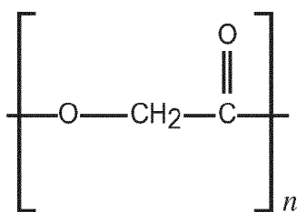
Poly(glycolide)
