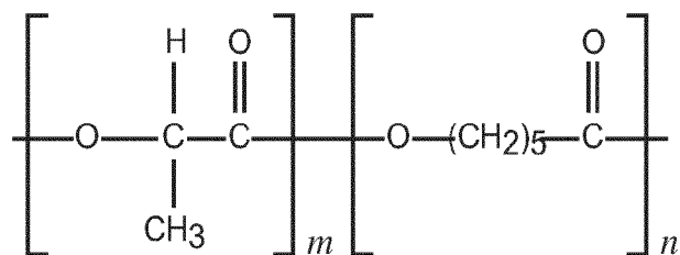
Poly(lactide-co-caprolactone)
