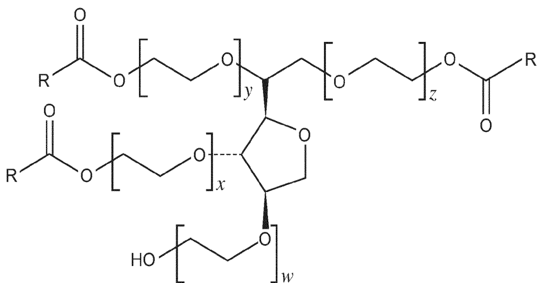
Polyoxyethylene sorbitan triester
