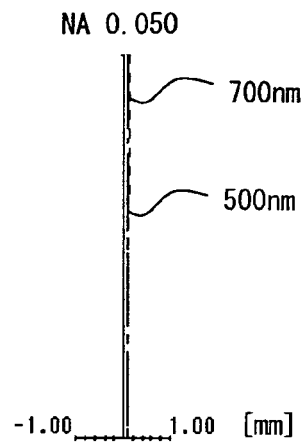
(a) AXIAL CHROMATIC ABERRATION OF COLLIMATOR LENS 26 + CONDENSING LENS 23
