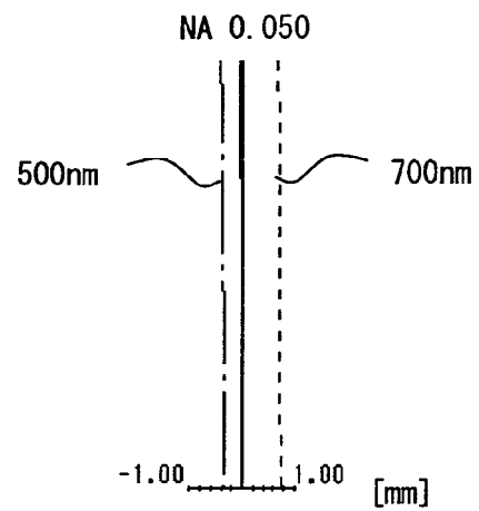
(b) AXIAL CHROMATIC ABERRATION OF COLLIMATOR LENS OF NORMAL DESIGN + CONDENSING LENS 23
