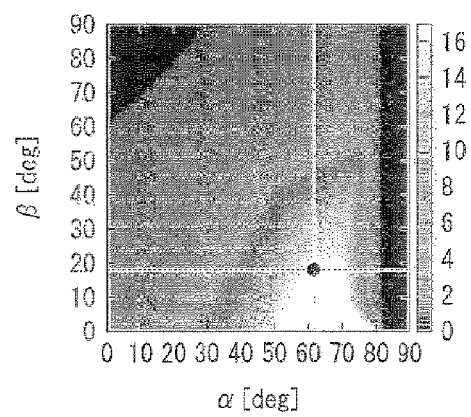
FIG.25B Max Size ( d = 4.1\text{mm} )
