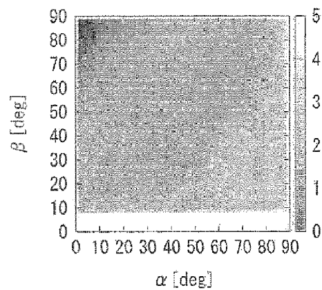
FIG.23B d = 3.0 \text{ mm}
