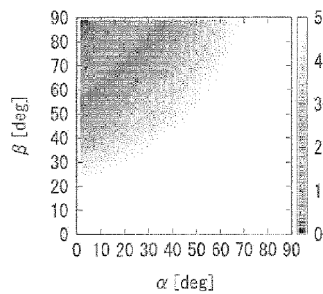
FIG.23D d = 7.0 \text{ mm}
