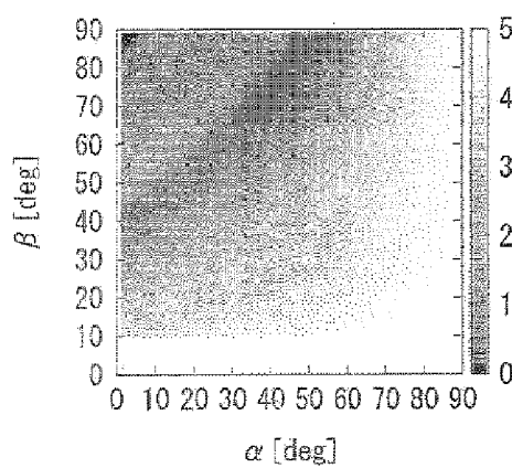
FIG.23C d = 5.0 \text{ mm}
