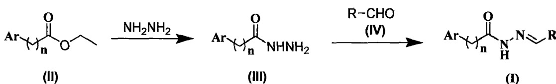
Scheme A The synthesis route of compound of general formula I
