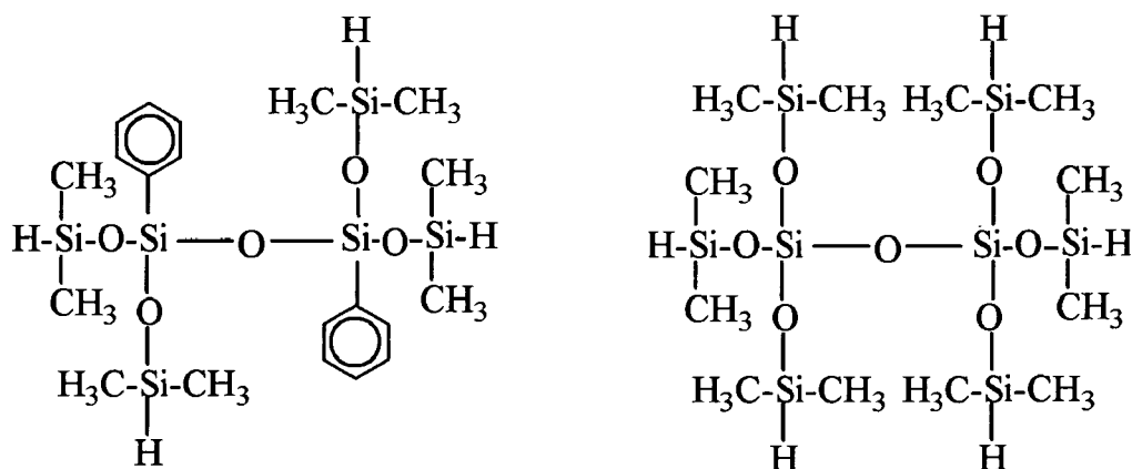
[Chemical Formula 2]
