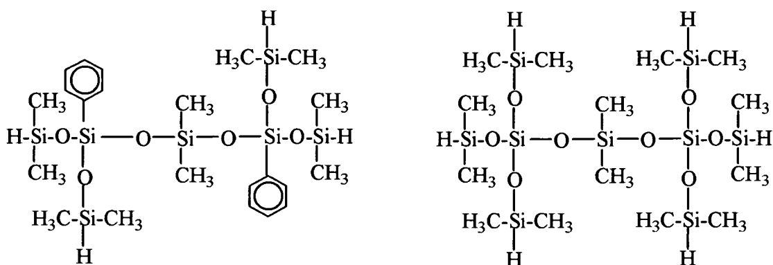
[Chemical Formula 3]
