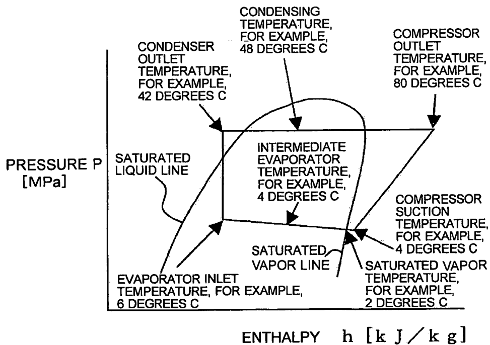
(b) WHEN CONSIDERING PRESSURE LOSS IN EVAPORATION
