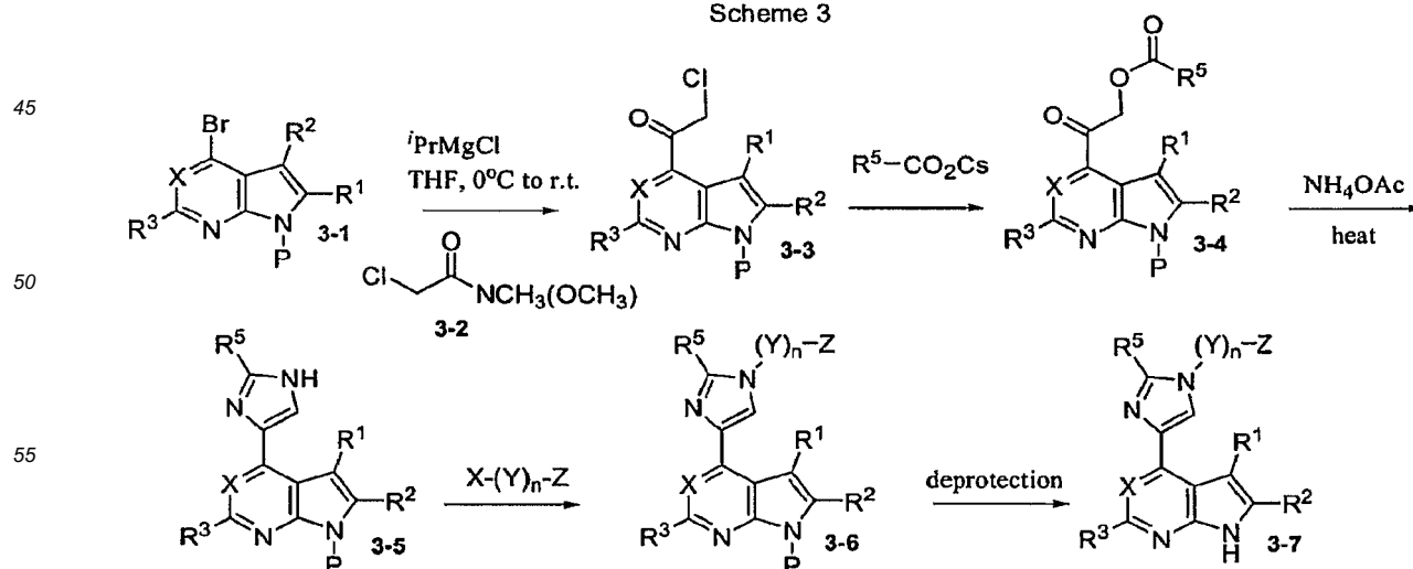
Scheme 3
