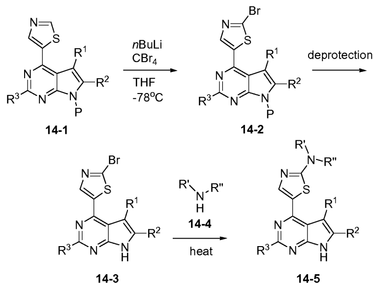
Scheme 14
