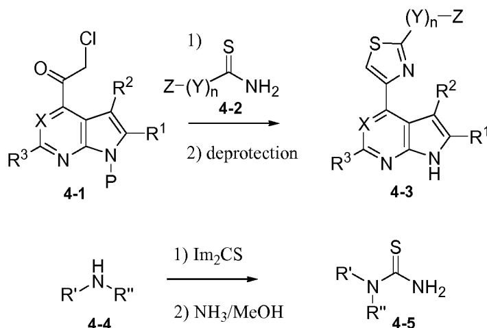
Scheme 4
