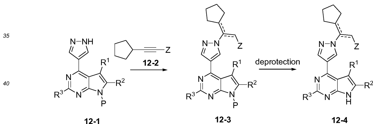
Scheme 12
