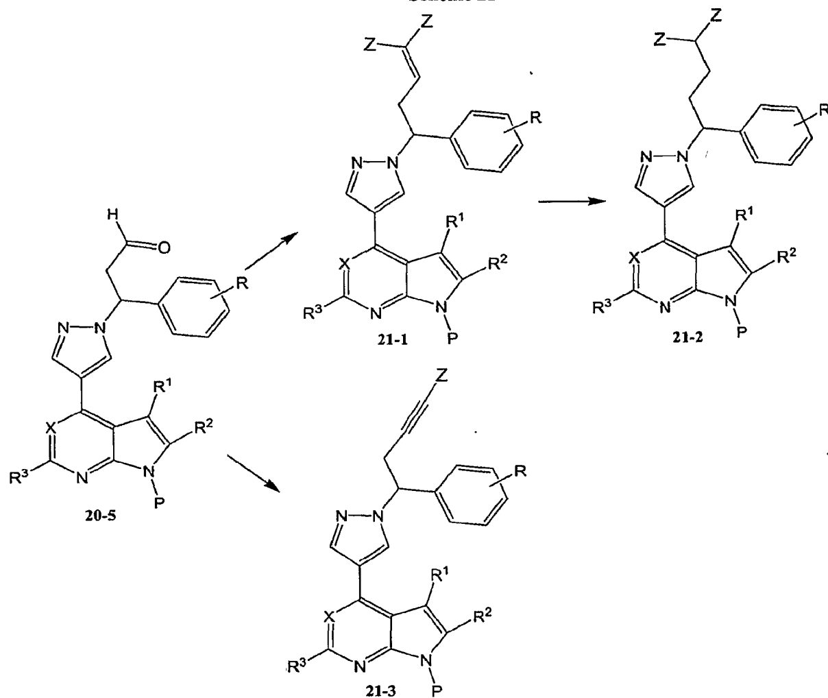
Scheme 21
