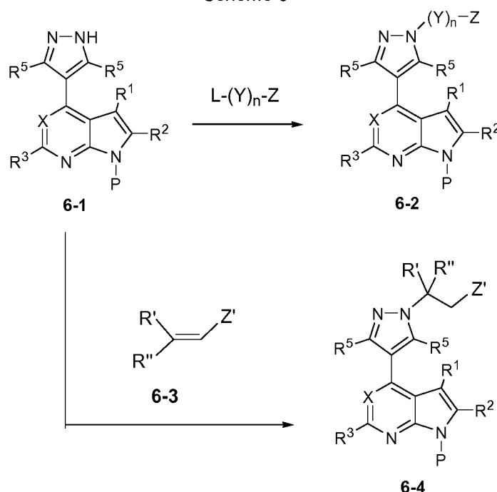
Scheme 6
