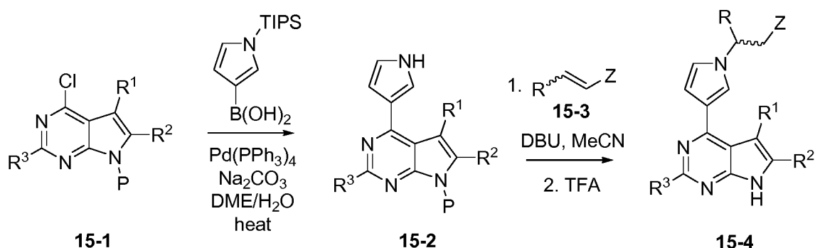
Scheme 15
