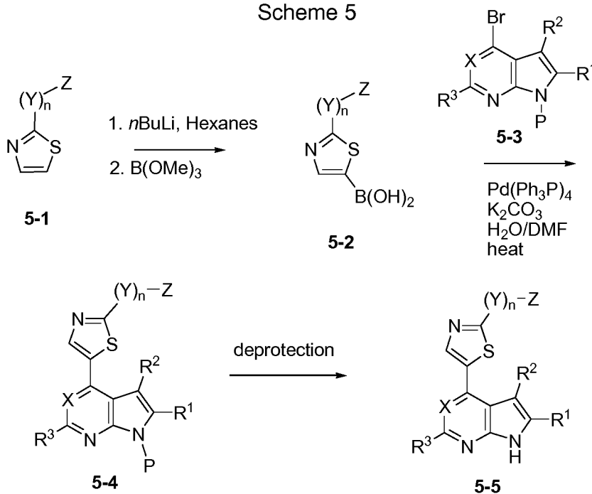
Scheme 5
