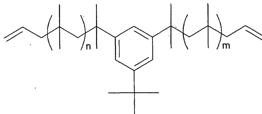
Allyl-PIB-Allyl
