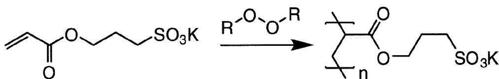
Reaction X
