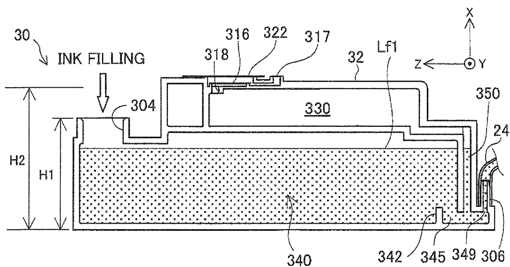
Fig.13C INK FILLING: EXCESS AMOUNT OF INK FILLING
