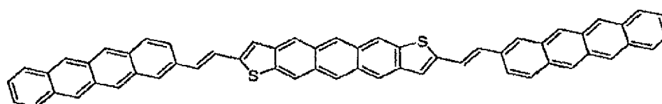
Compound 30
