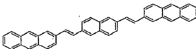
Compound 13
