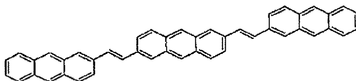
Compound 8
