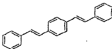
Compound 39
