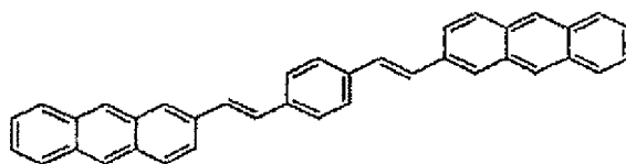
Compound 16
