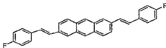
Compound 2
