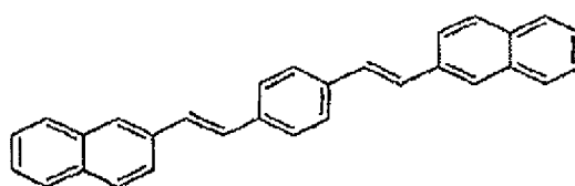
Compound 40
