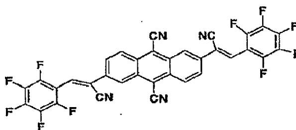
Compound 46
