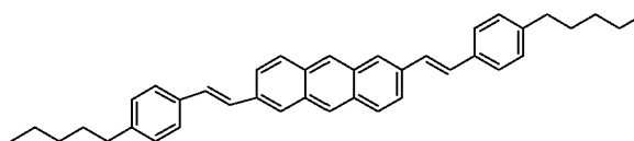
Compound 3
