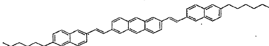
Compound 4
