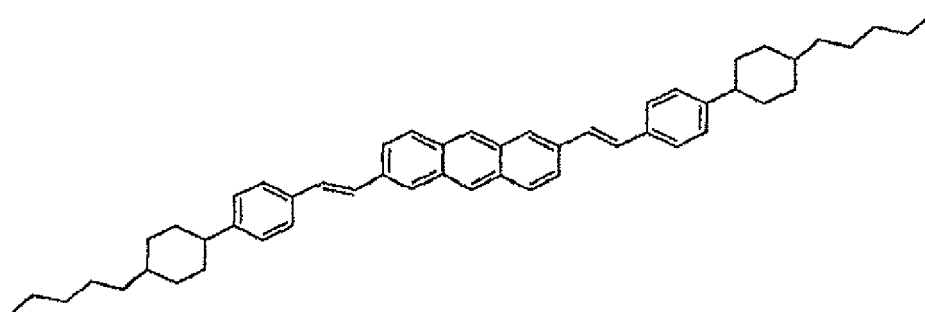
Compound 43
