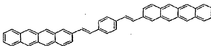
Compound 42
