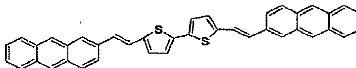
Compound 38
