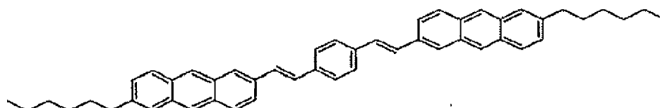
Compound 17
