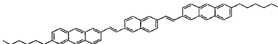
Compound 15
