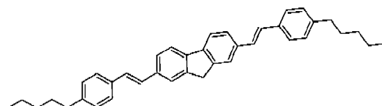
Compound 49
