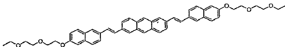
Compound 8
