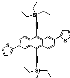
Compound 84
