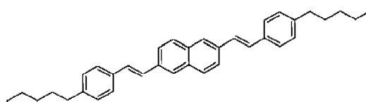
Compound 48
