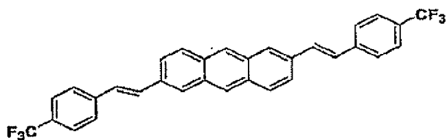
Compound 45
