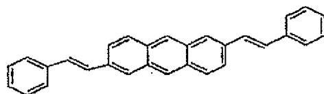
Compound 1
