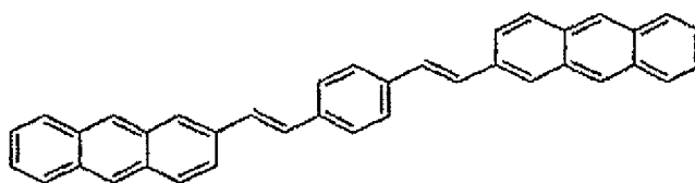
Compound 41
