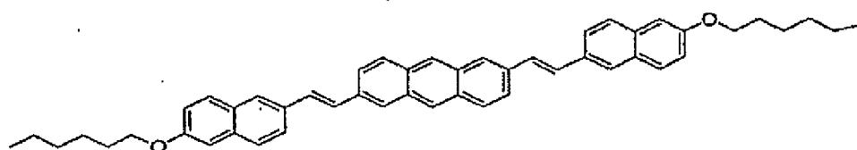
Compound 6
