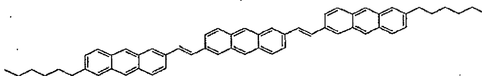
Compound 9
