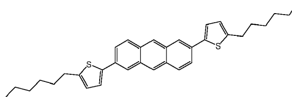
Compound 77.
