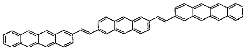
Compound 10
