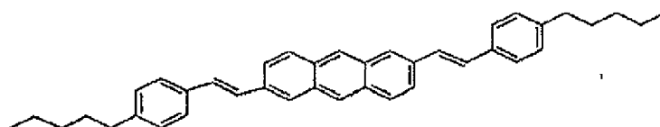
Compound 3
