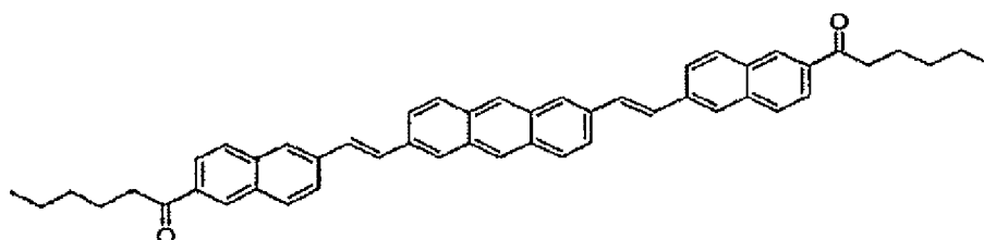
Compound 5
