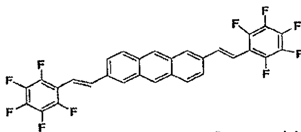
Compound 44
