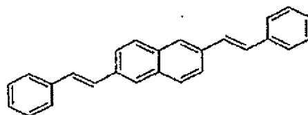
Compound 47
