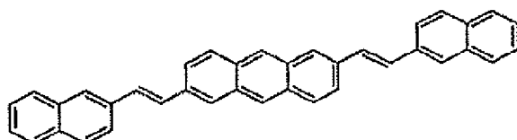
Compound 3
