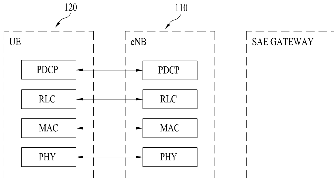
(b) USER-PLANE PROTOCOL STACK
