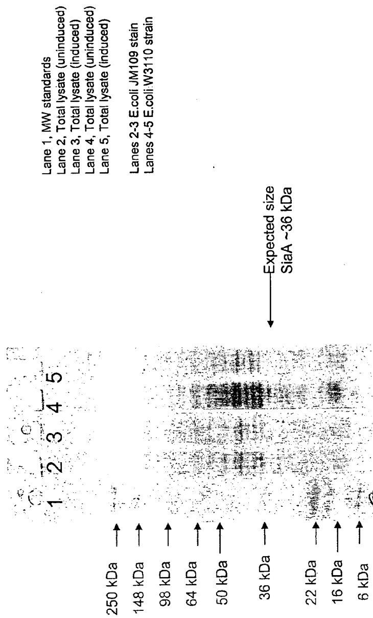
Figure 28: Induced SiaA expression in E.coli
