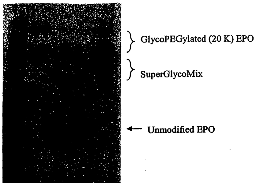
Figure 5. GlycoPEGylation (20 K) of EPO
