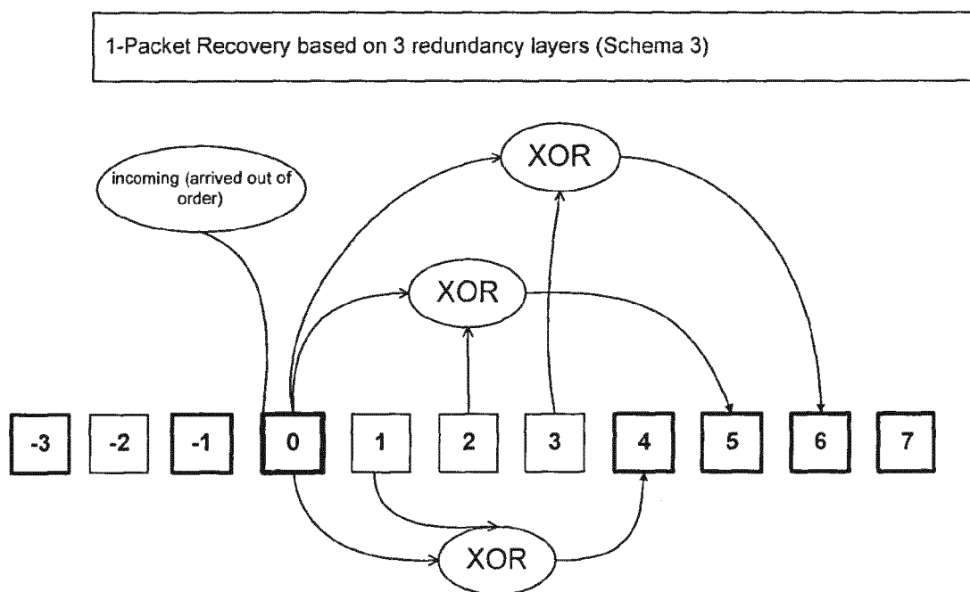
Offset based 1-Packet Recovery Schema 3
