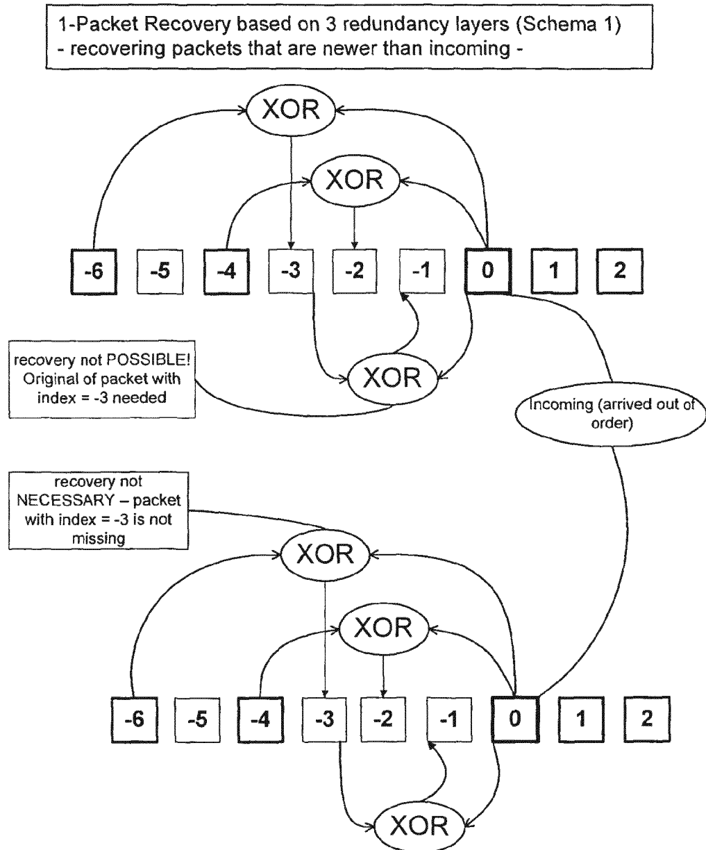
Offset based 1-Packet Recovery Schema 1
