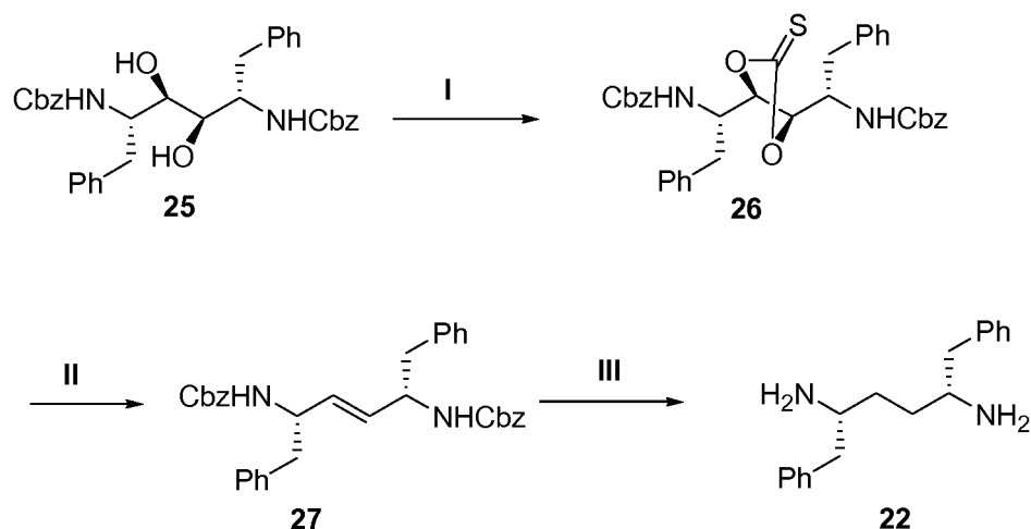
Scheme 12
