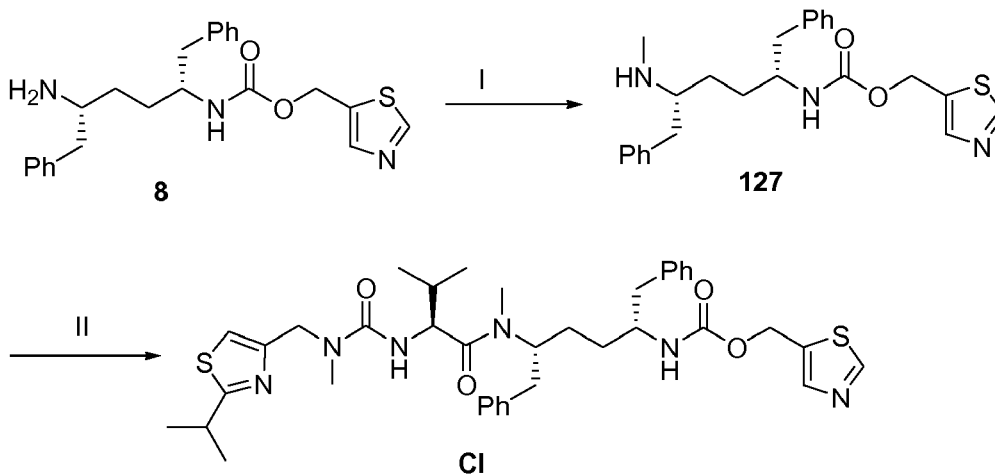
Scheme 72
