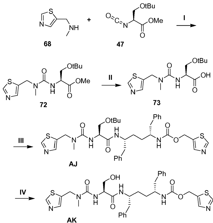
Scheme 30
