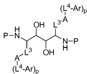
Analog of Compound 25
