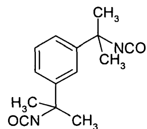
TMXDI NCO-content(w/w)~34.4
