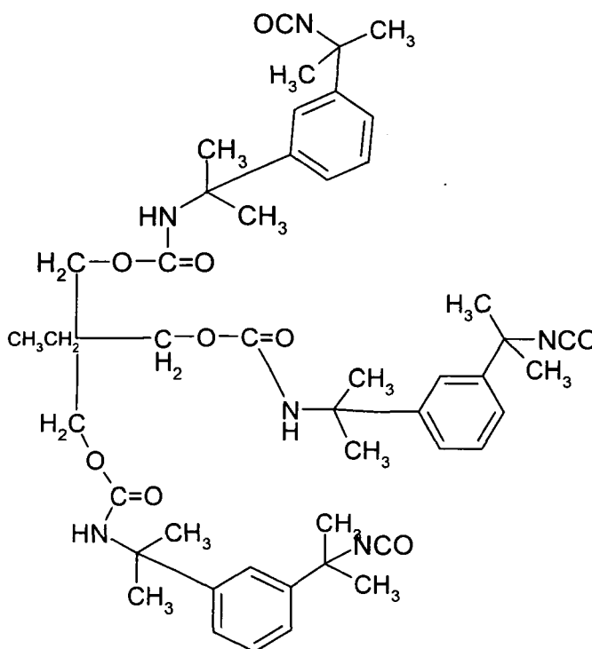
Cythane 3174-Pre-polymer in Butyl Acetate NCO- content(w/w)~10.2
