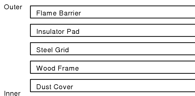
Fig. 3: Foundation in order from outer to inner
