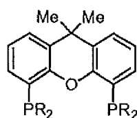
(XXX) R = Ph (XXXI) R = 3,5-( \text{CF}_3 ) 2 Ph
