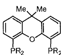
(XXX) R = Ph (XXXI) R = 3,5-(CF_3)_2Ph
