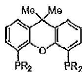
(XXX) R = Ph (XXXI) R = 3,5-(CF 3 ) 2 Ph
