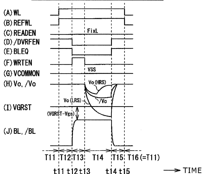
WORKING EXAMPLE 1-1 (RESET & DIRECT VERIFY OPERATION)
