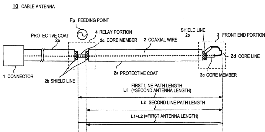
EXAMPLE OF CONFIGURATION OF CABLE ANTENNA
