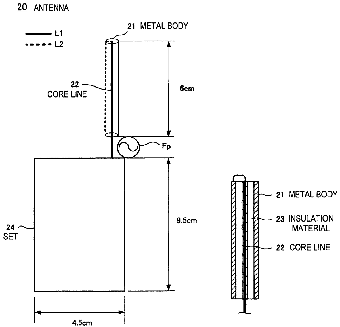
EXAMPLE OF CONFIGURATION OF ANTENNA MOUNTED ON PORTABLE TERMINAL
