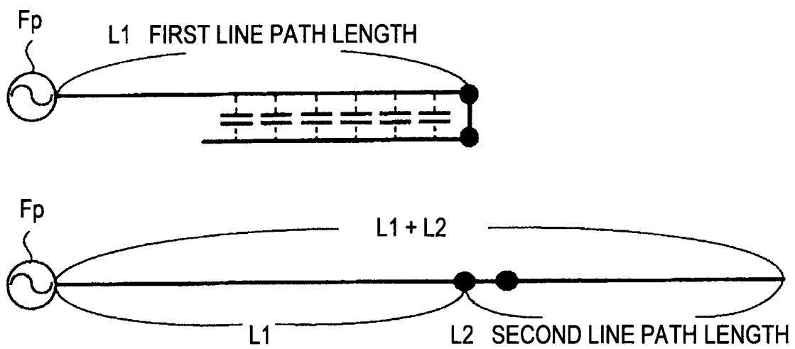
DIAGRAM FOR PRINCIPLE OF CABLE ANTENNA
