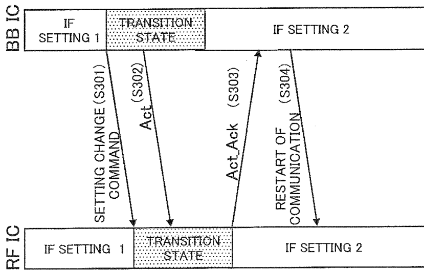
FIG. 4A EXEMPLARY EMBODIMENT OF THE PRESENT INVENTION
