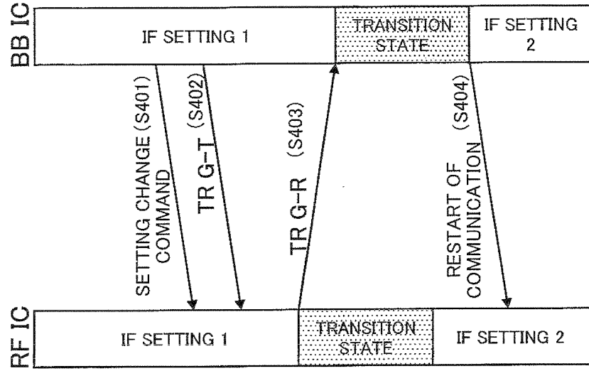
FIG. 4B BACKGROUND ART (EXAMPLE OF DigRF v4)
