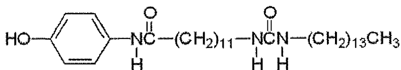
Structural Formula (1)
