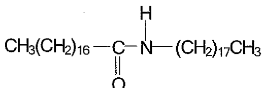
Structural Formula (3)
