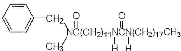
Structural Formula (2)
