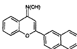
Example 74 (reference) inactive on mGluR4 up to 100 μM
