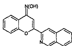
Example 1 mGluR4 PAM EC 50 < 0.5 μM
