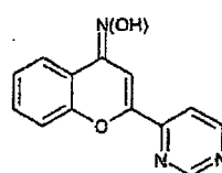
Example 80 (reference) inactive on mGluR4 up to 100 μM
