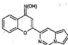
Example 63 mGluR4 PAM EC 50 < 0.5 μM
