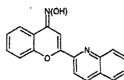
Example 79 (reference) inactive on mGluR4 up to 100 μM
