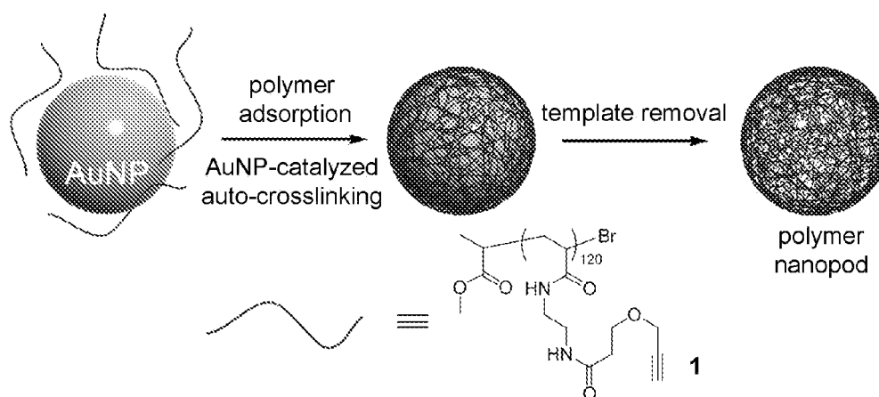
Scheme 1. Synthesis of polyvalent propargyl ether nanoconjugates.
