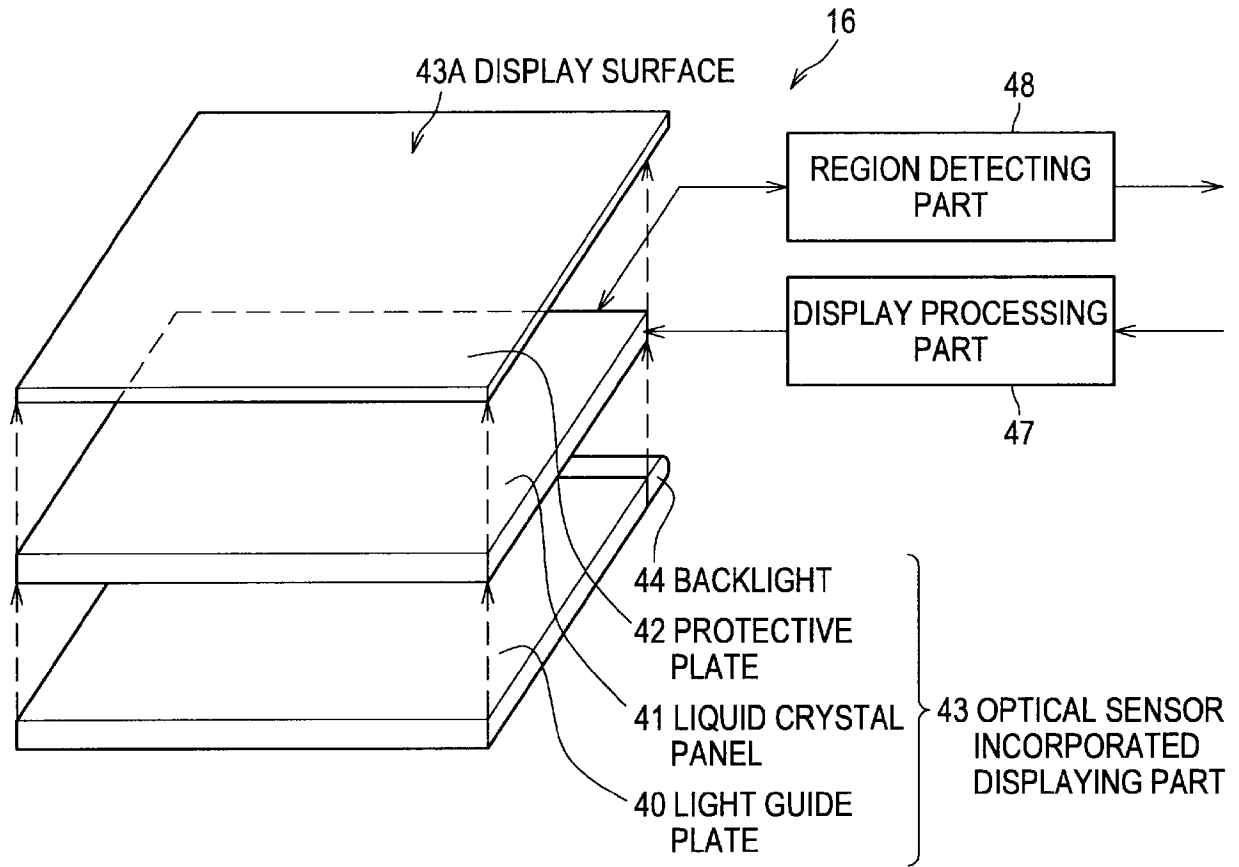
STRUCTURE OF OPERATION SCREEN
