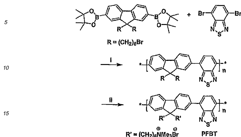
Scheme 1. Reaction conditions: i) 2M K_2CO_3 , toluene, Pd(PPh_3)_4 ; ii) NMe_3 , THF/ H_2O .
