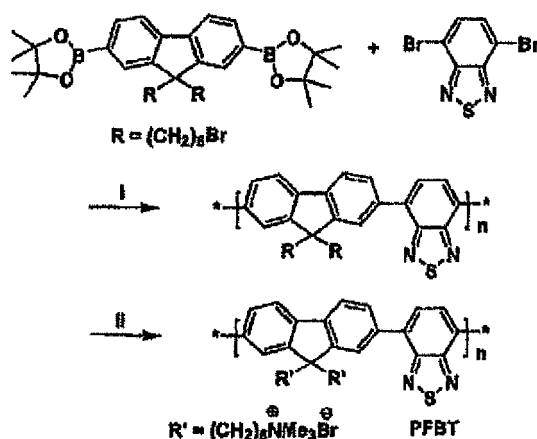
Scheme 1. Reaction conditions: i) 2M K 2 CO 3 , toluene, Pd(PPh 3 ) 4 ; ii) NMe 3 , THF/H 2 O.
