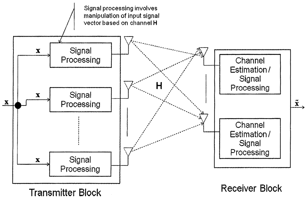
Figure 2 (Prior Art)
