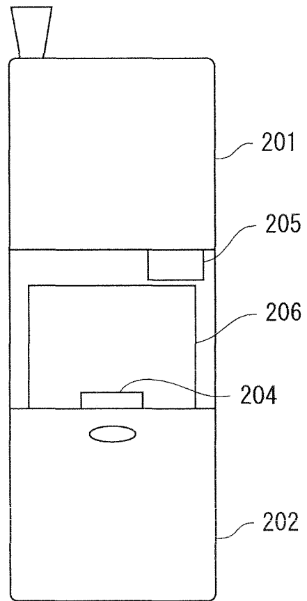
MOBILE TERMINAL DEVICE WHOSE BATTERY COVER IS MOVED
