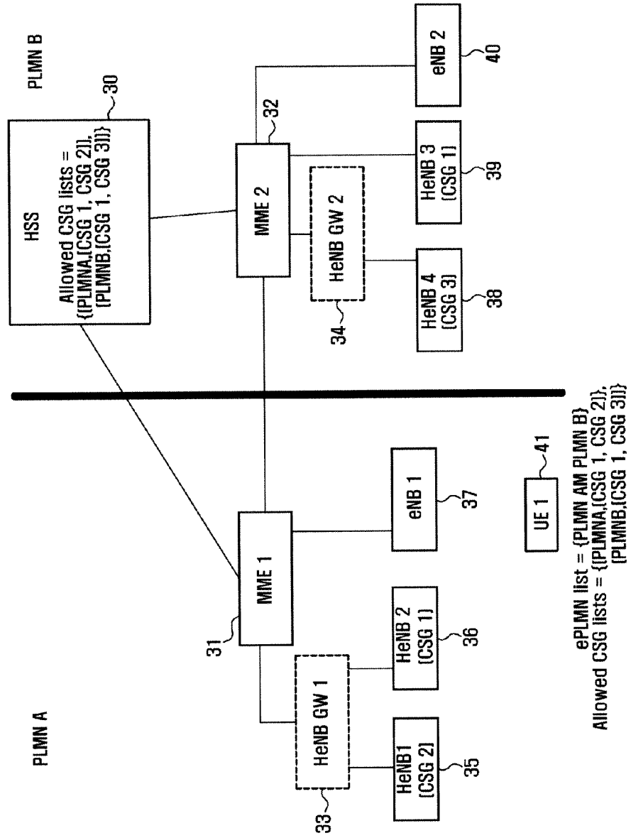
FIG. 3 (RELATED ART)
