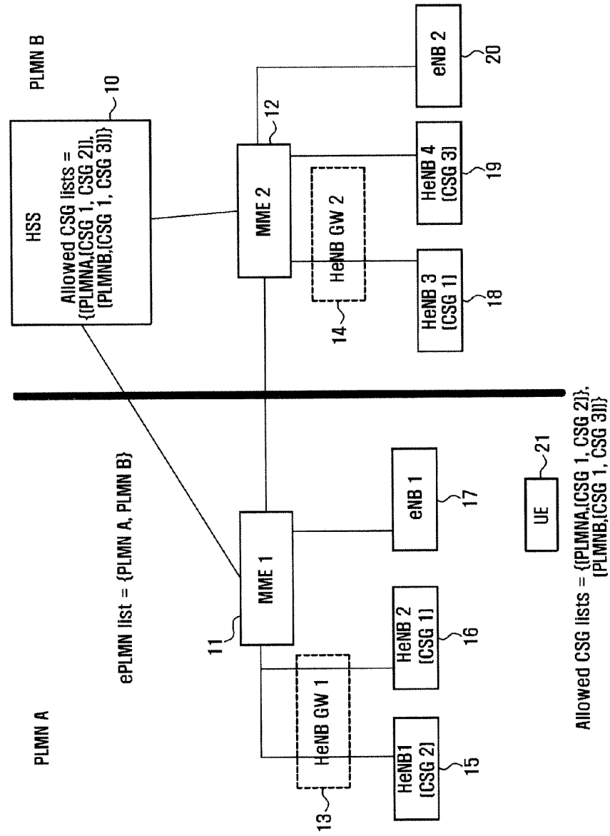
FIG. 1 (RELATED ART)
