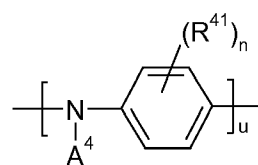
(VIb),
