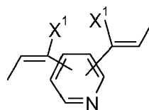
(VIb),
