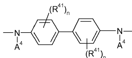
(VIe), or
