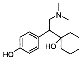
O-desmethylvenlafaxine
