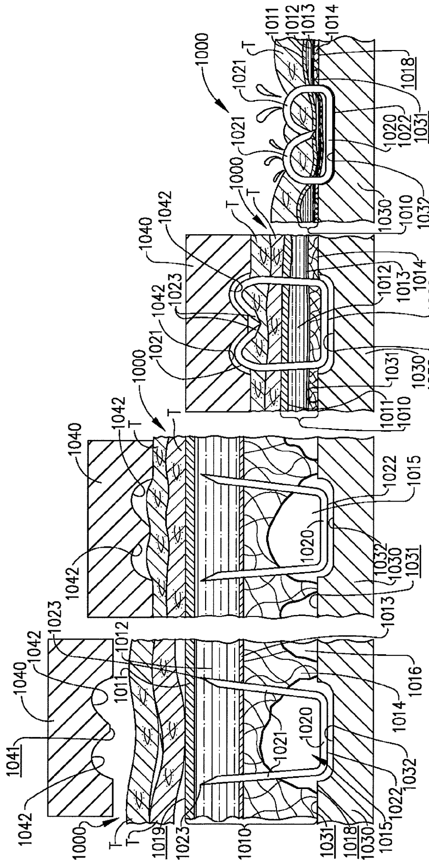
JAW OPEN JAW CLOSED COMPLETELY FORMED FIG. 18A FIG. 18B FIG. 18D
