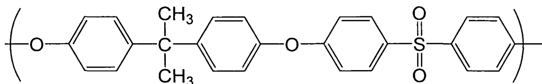
[Chemical Formula 1]
