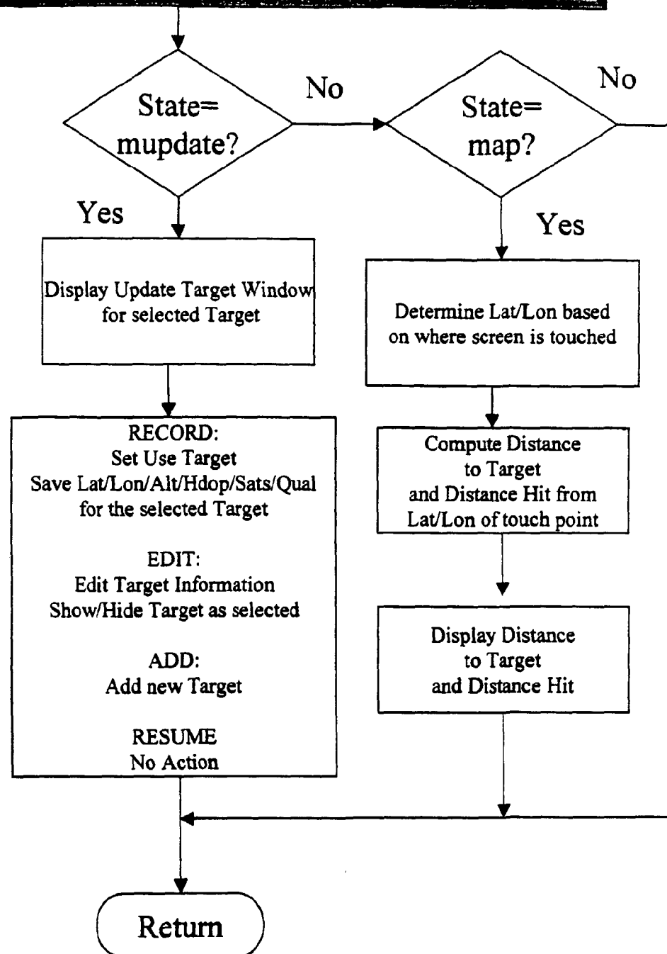
Fig. 4 - Process Pen Down Event
