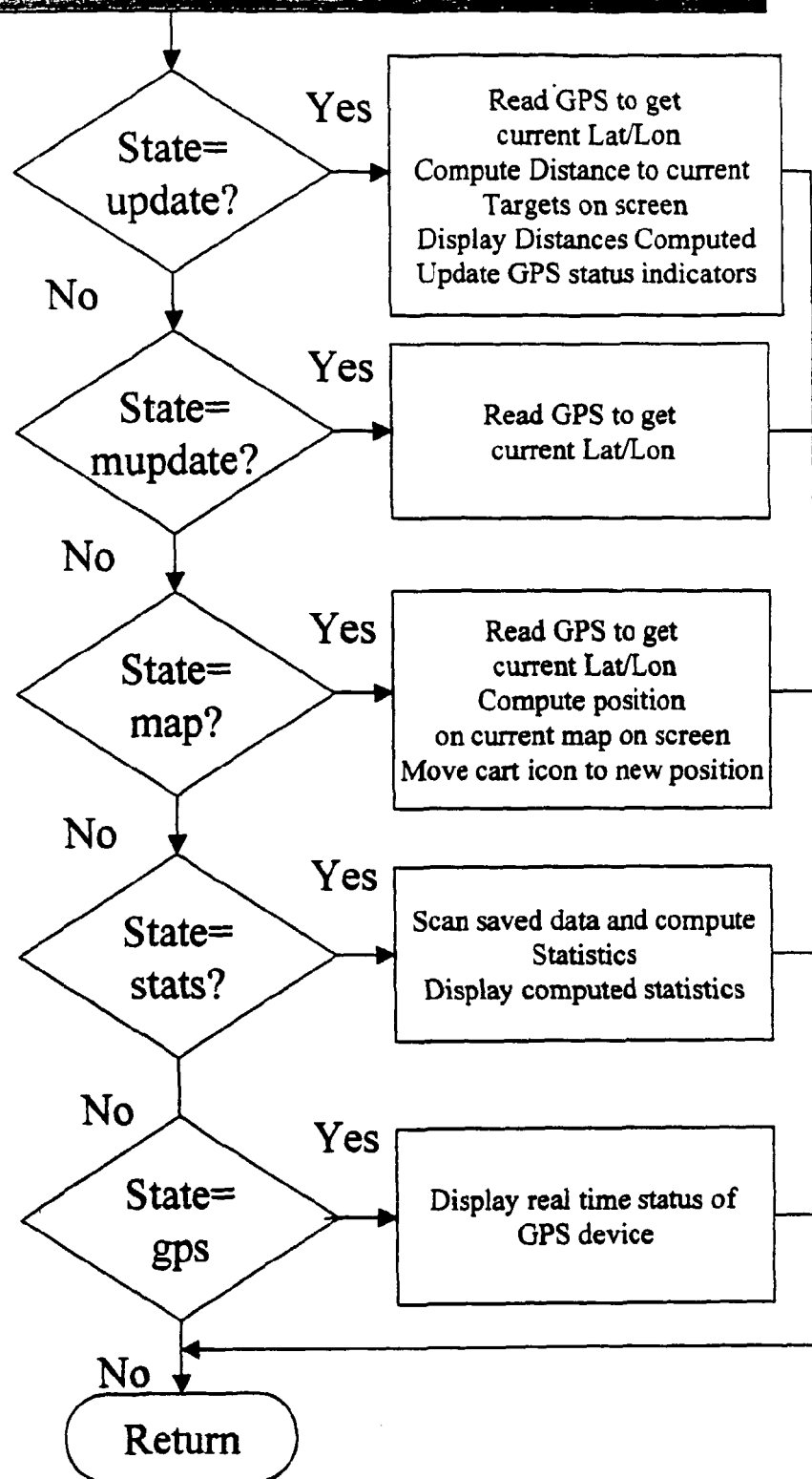
Fig. 7 - Process State Action
