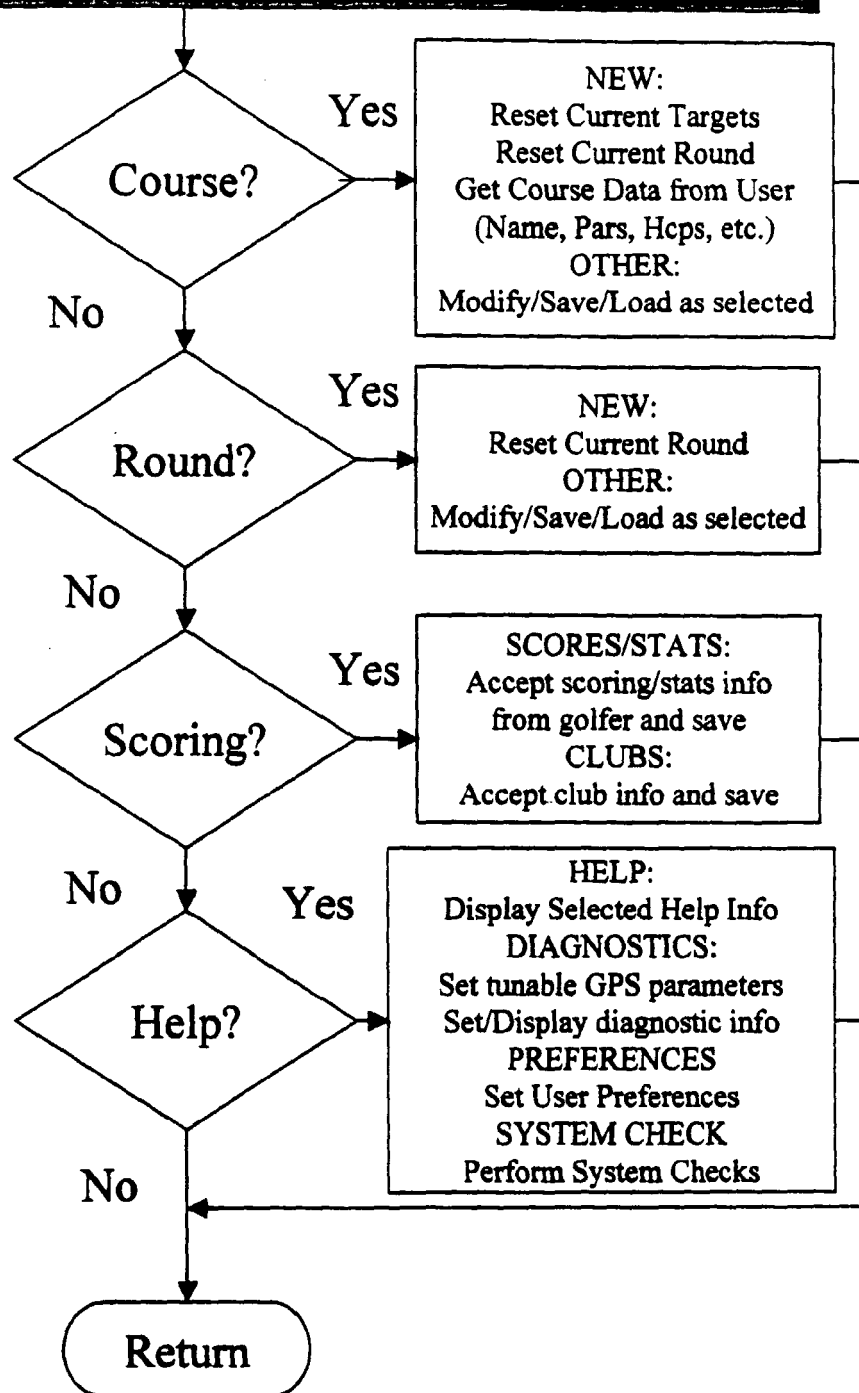
Fig. 3 - Process Menu Event
