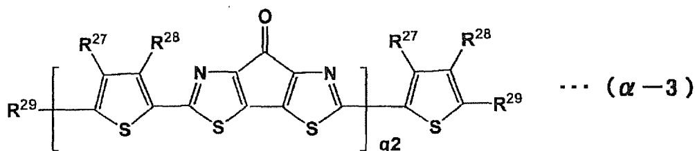
[Chemical Formula 50]
