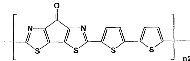
[Chemical Formula 73]
