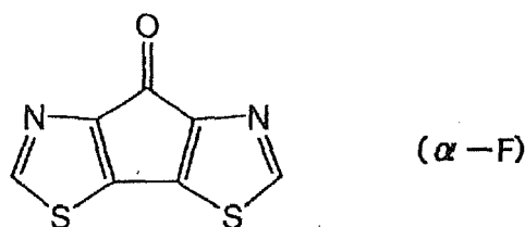
[Chemical Formula 107]
