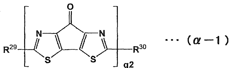
[Chemical Formula 48]
