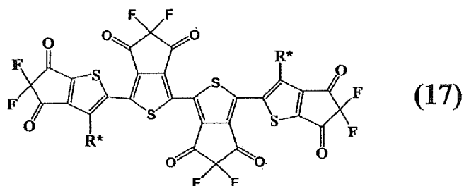
[Chemical Formula 29]
