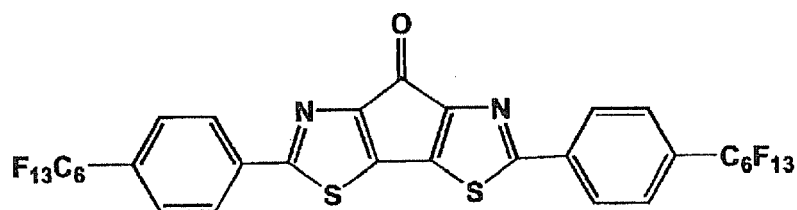
[Chemical Formula 66]
