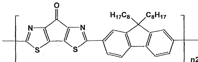
[Chemical Formula 73]
