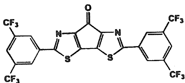
[Chemical Formula 60]
