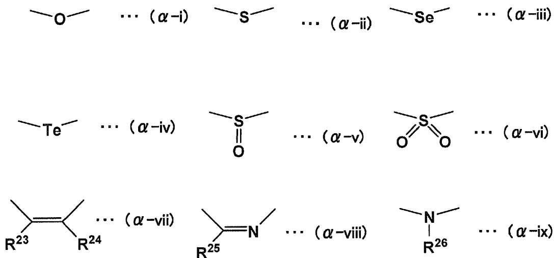
[Chemical Formula 9]
