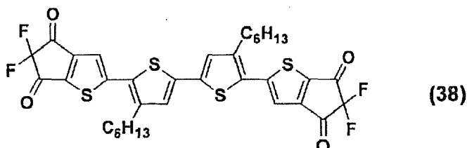
[Chemical Formula 93]
