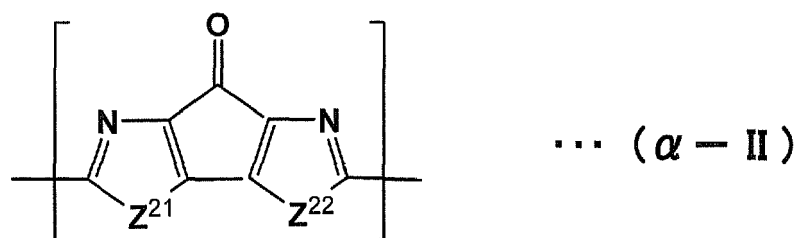
[Chemical Formula 13]
