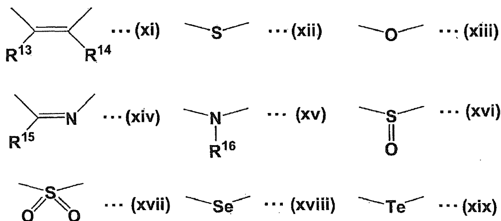
[Chemical Formula 41]
