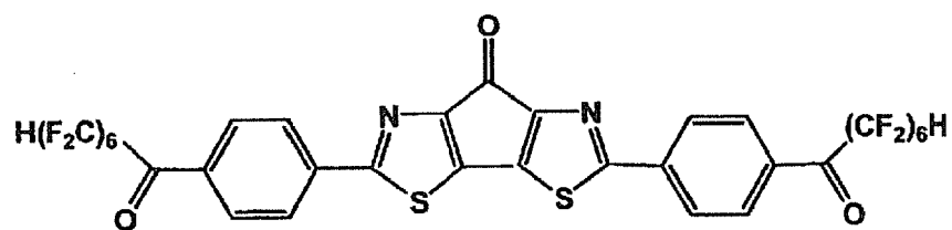
[Chemical Formula 65]
