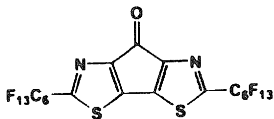
[Chemical Formula 55]
