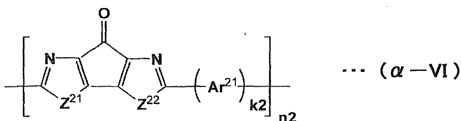
[Chemical Formula 46]
