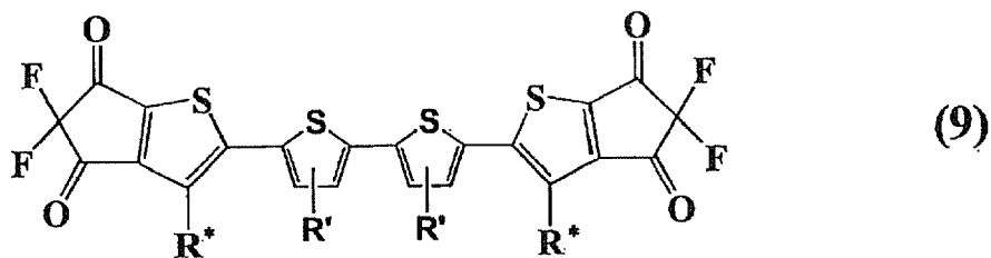
[Chemical Formula 20]
