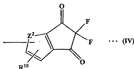
[Chemical Formula 40]
