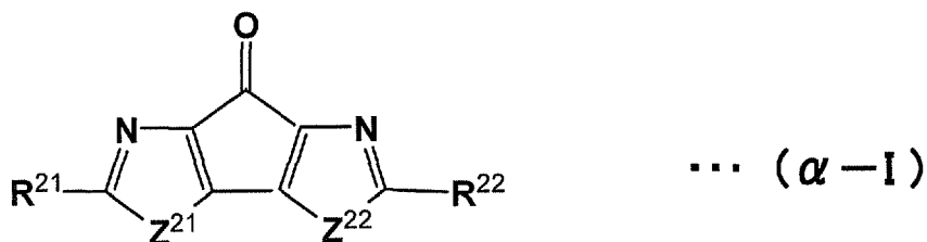
[Chemical Formula 8]
