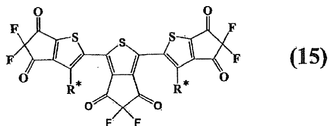
[Chemical Formula 26]
