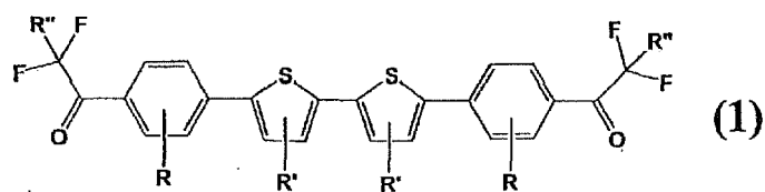
[Chemical Formula 12]
