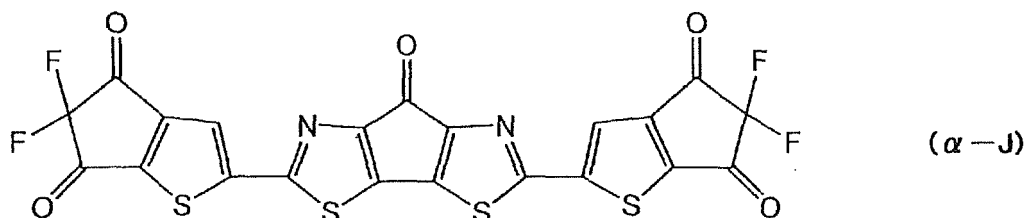
[Chemical Formula 111]
