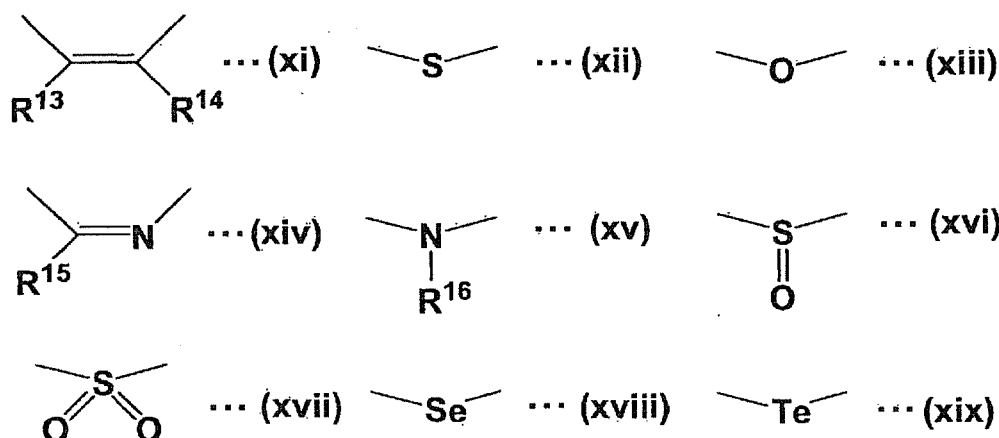
[Chemical Formula 10]
