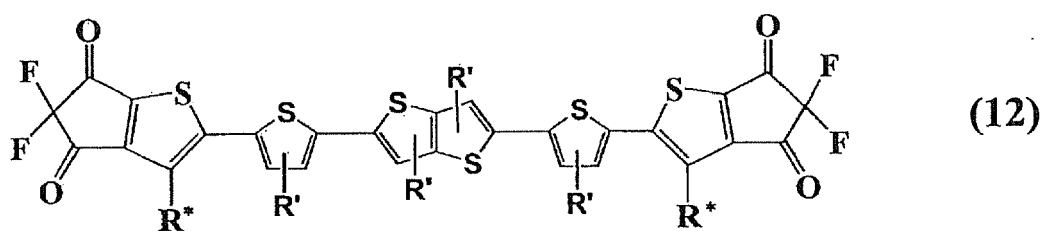
[Chemical Formula 23]
