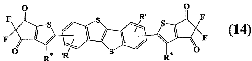
[Chemical Formula 26]
