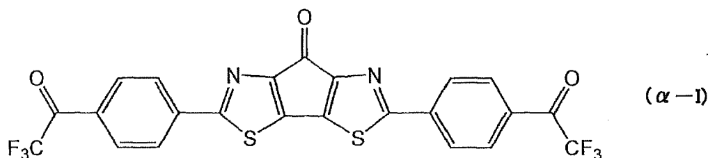
[Chemical Formula 110]
