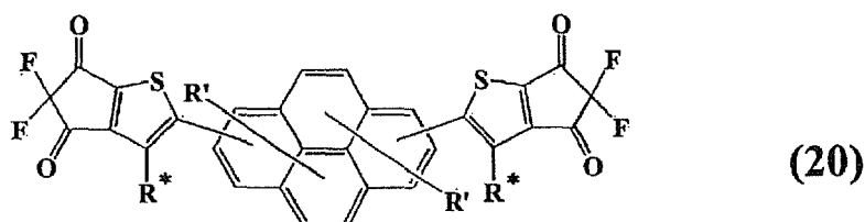
[Chemical Formula 31]
