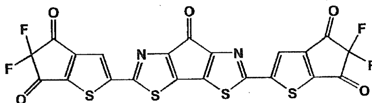
[Chemical Formula 69]
