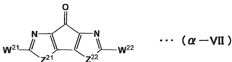
[Chemical Formula 77] W^{21} -Ar 21 - W^{22} ( \alpha -VIII)
