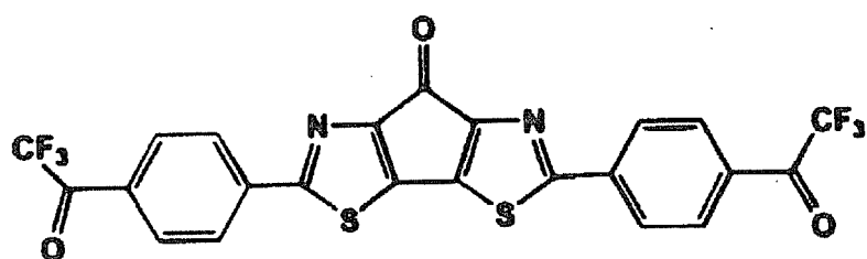
[Chemical Formula 59]
