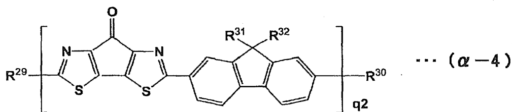
[Chemical Formula 51]
