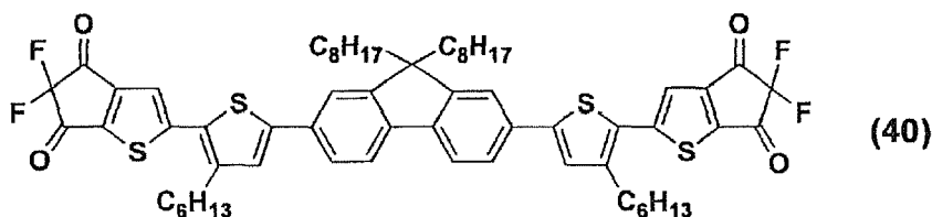
[Chemical Formula 95]
