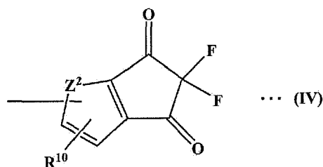
[Chemical Formula 11]
