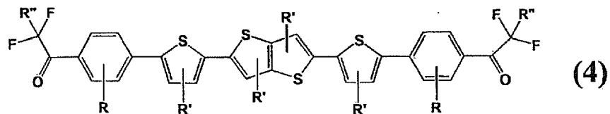
[Chemical Formula 15]
