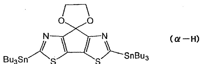
[Chemical Formula 109]
