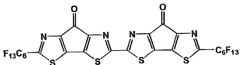
[Chemical Formula 62]
