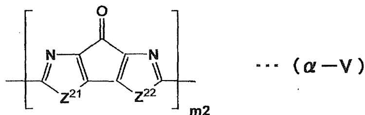
[Chemical Formula 45]
