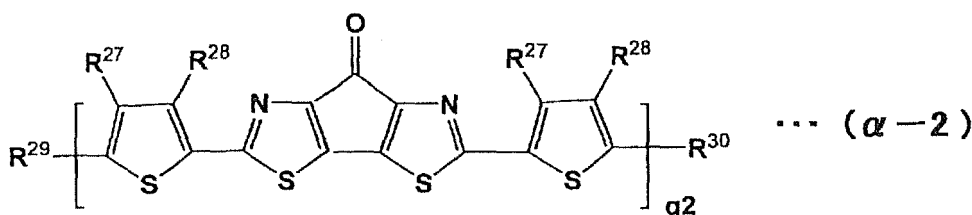
[Chemical Formula 49]
