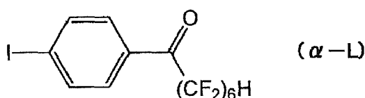
[Chemical Formula 112]
