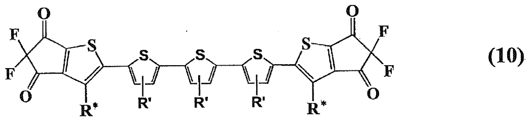
[Chemical Formula 21]
