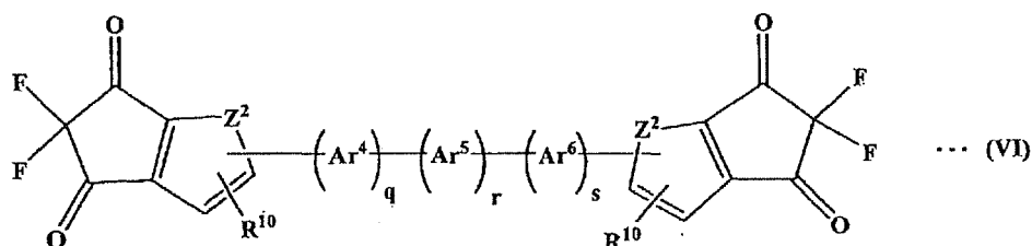
[Chemical Formula 11]
