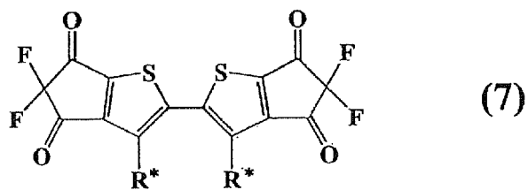
[Chemical Formula 18]
