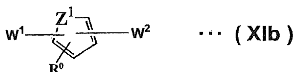
[Chemical Formula 37]
