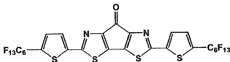
[Chemical Formula 67]
