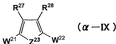
[Chemical Formula 78]
