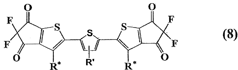
[Chemical Formula 19]
