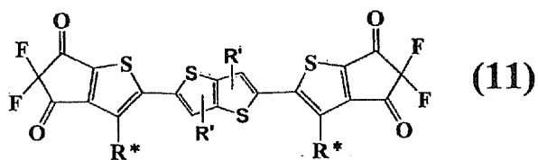
[Chemical Formula 22]
