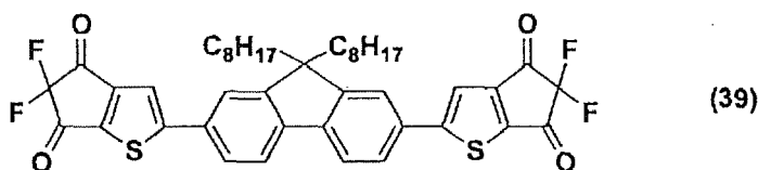
[Chemical Formula 94]
