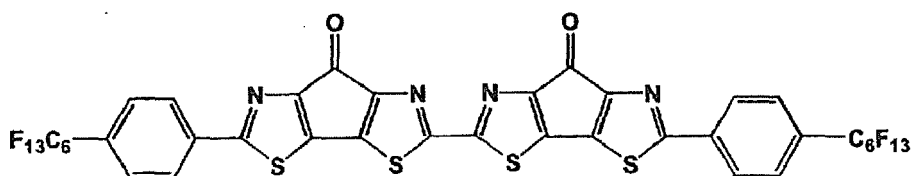
[Chemical Formula 70]
