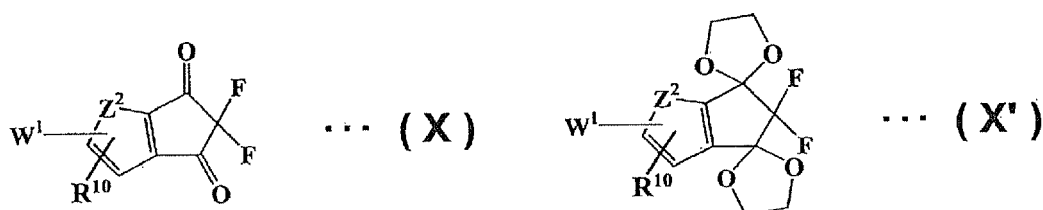
[Chemical Formula 35]
