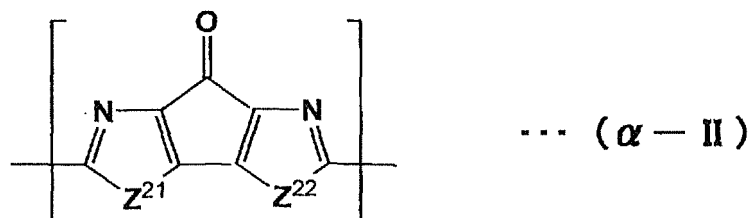
[Chemical Formula 4]
