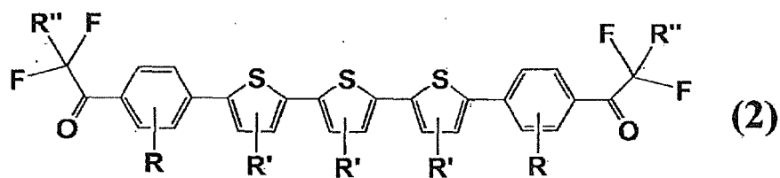
[Chemical Formula 14]
