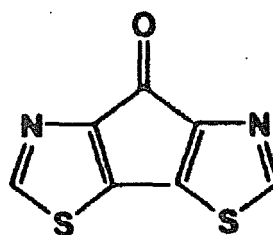
[Chemical Formula 53]
