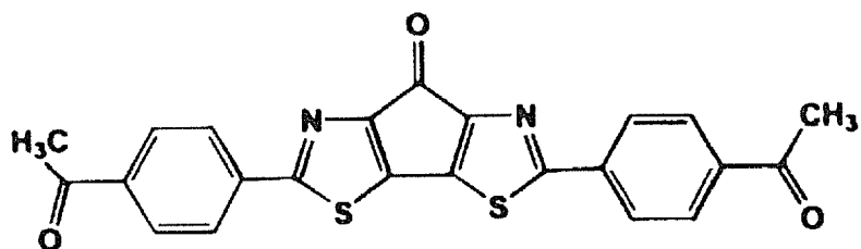
[Chemical Formula 58]
