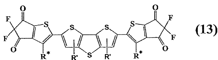
[Chemical Formula 25]
