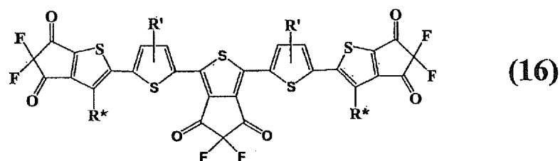
[Chemical Formula 27]
