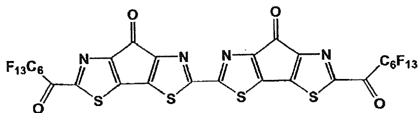
[Chemical Formula 63]
