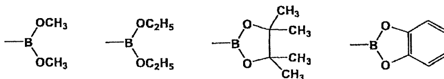
[Chemical Formula 47]
