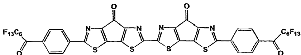
[Chemical Formula 71]
