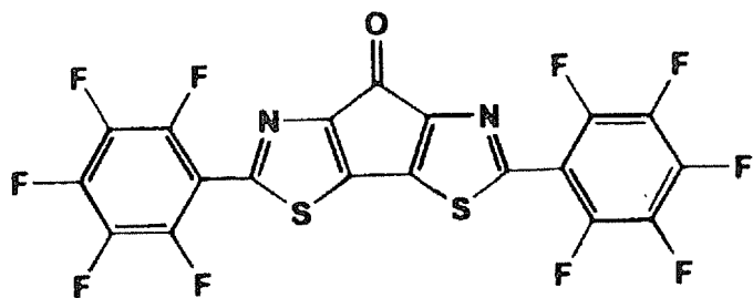
[Chemical Formula 57]
