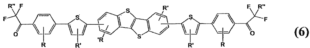
[Chemical Formula 17]
