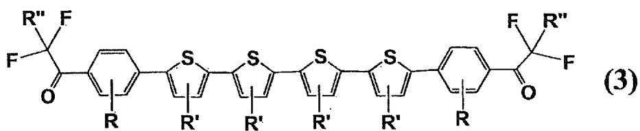
[Chemical Formula 15]
