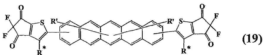
[Chemical Formula 31]
