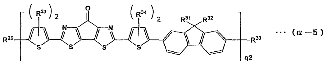
[Chemical Formula 52]
