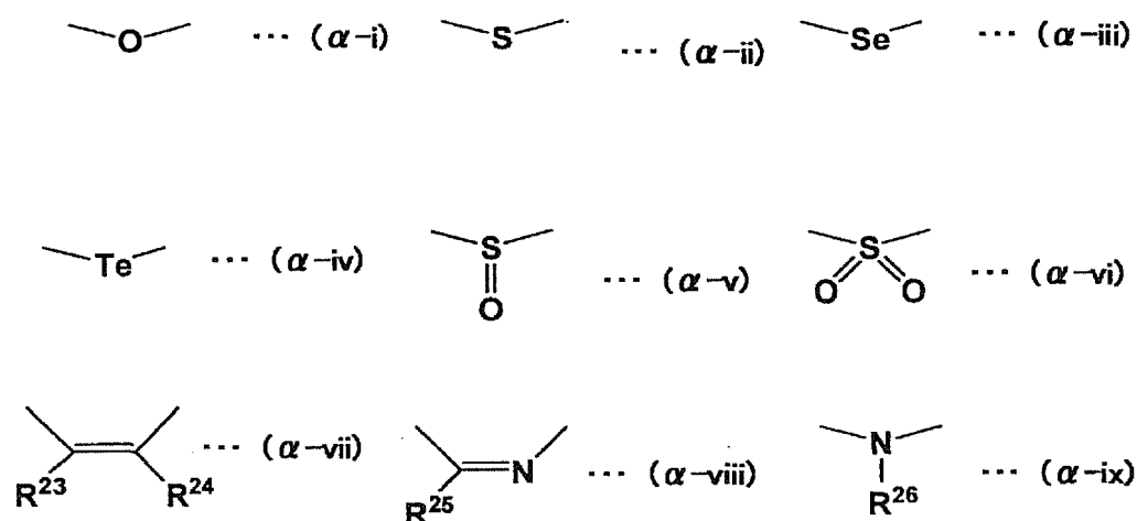
[Chemical Formula 5]
