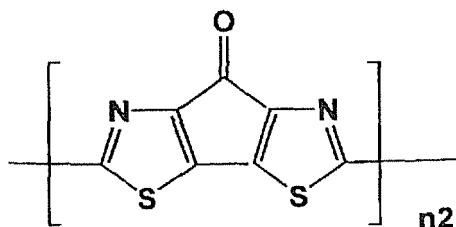
[Chemical Formula 71]
