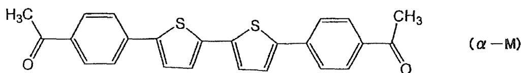
[Chemical Formula 114]
