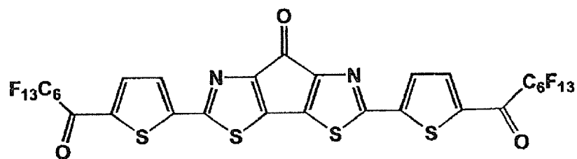
[Chemical Formula 67]
