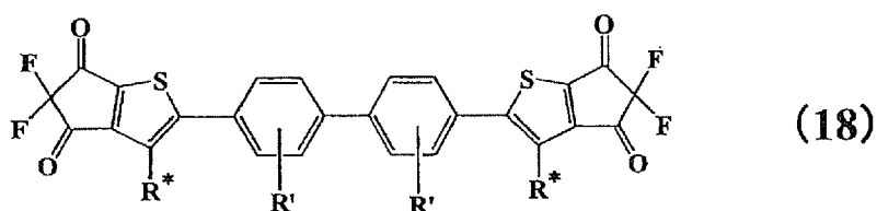
[Chemical Formula 30]
