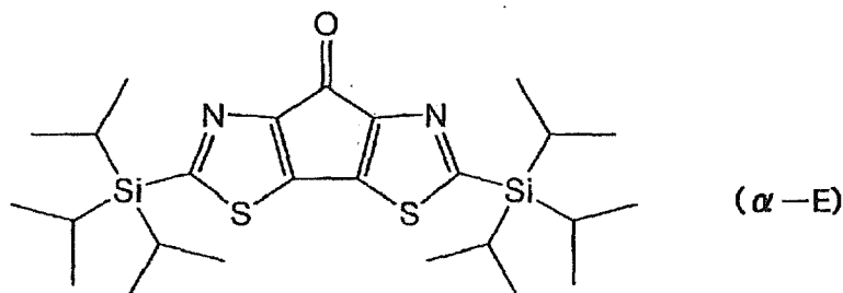
[Chemical Formula 106]
