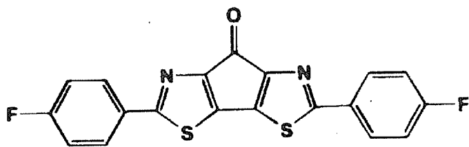
[Chemical Formula 57]
