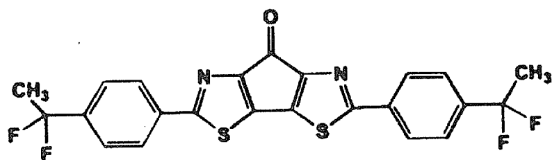
[Chemical Formula 61]
