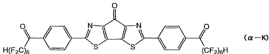
[Chemical Formula 113]
