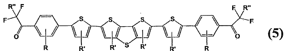
[Chemical Formula 16]
