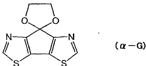
[Chemical Formula 108]
