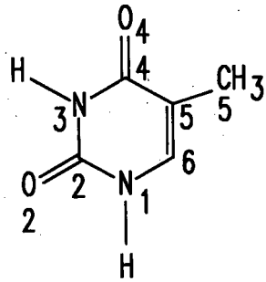
Thymine (Thy)
