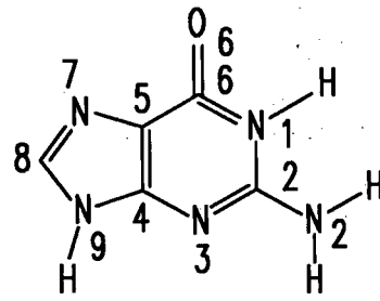
Guanine (Gua)
