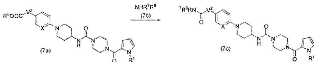
Reaction Scheme 7
