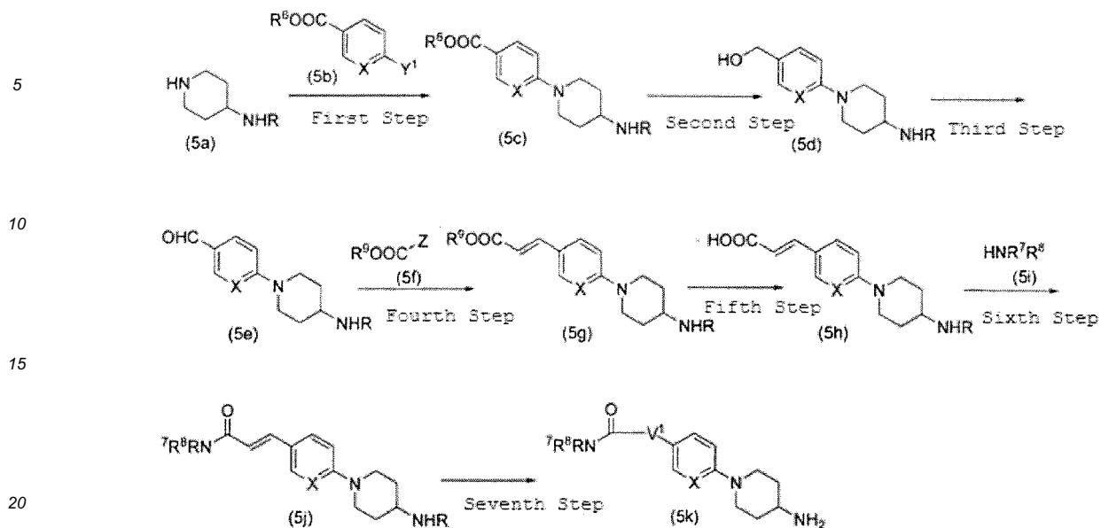
Reaction Scheme 5
