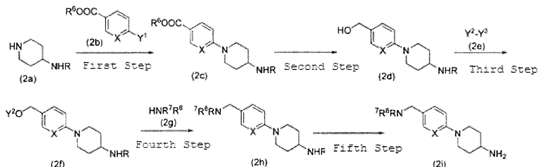
Reaction Scheme 2
