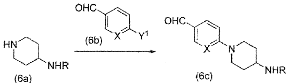
Reaction Scheme 6
