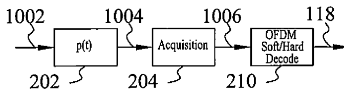
Figure 10 (Related Art)
