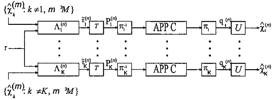
Iterative multiuser decoder with linear multiuser estimation
