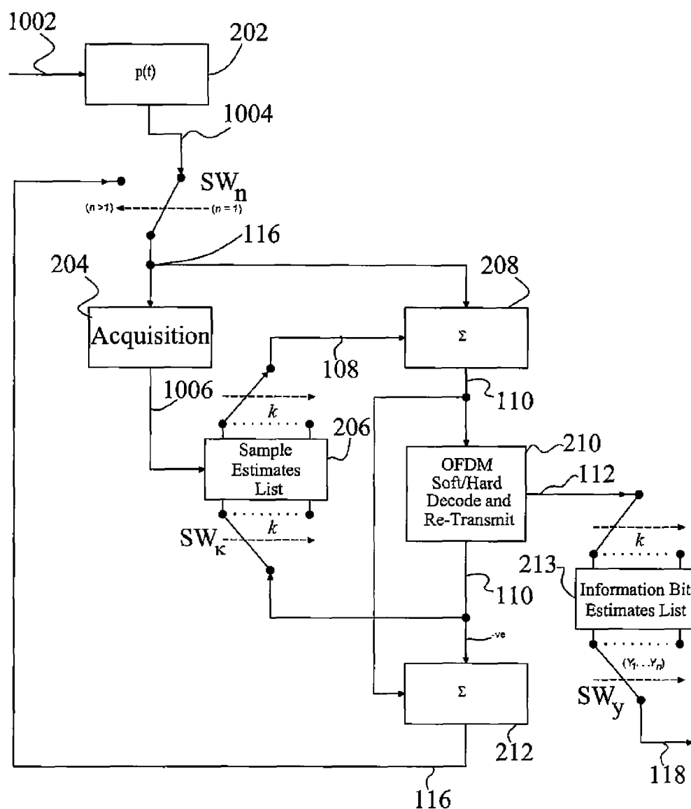
Iterative Interference Canceling Receiver Structure
