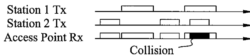
Figure 2 (Related Art)
