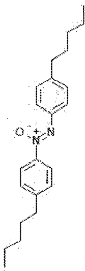
Formula 5
