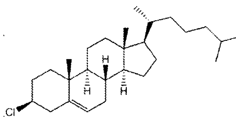
Formula 4
