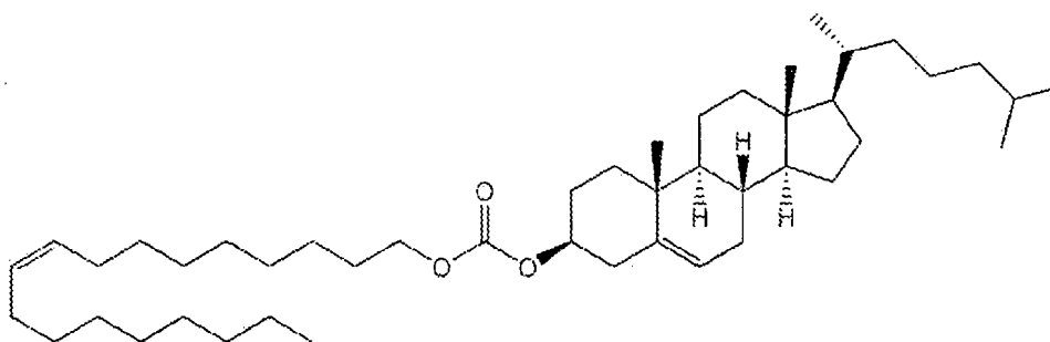
Formula 2
