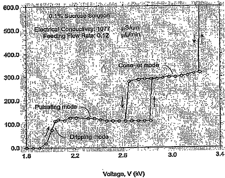
Typical current vs. Voltage Curve for Electrospray
