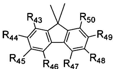
[Chemical Formula 4]
