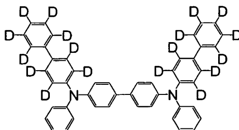
[Chemical Formula 63]
