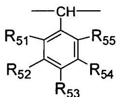
[Chemical Formula 6]
