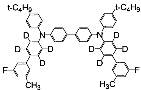
[Chemical Formula 29]
