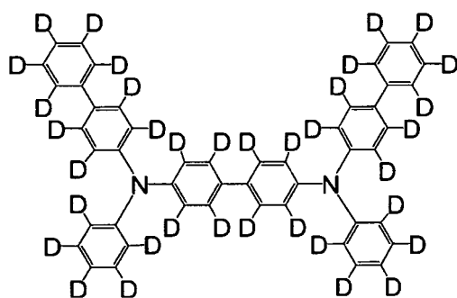
[Chemical Formula 23]
