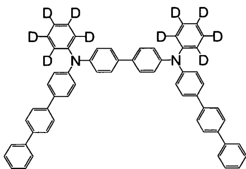
[Chemical Formula 26]
