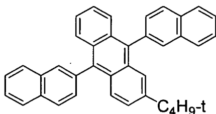
[Chemical Formula 69]
