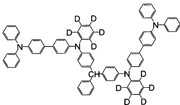
[Chemical Formula 62]
