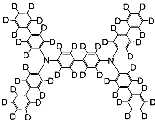
[Chemical Formula 37]
