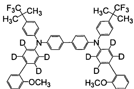
[Chemical Formula 30]
