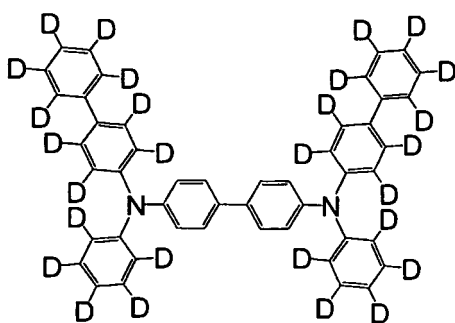
[Chemical Formula 22]
