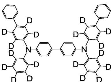
[Chemical Formula 21]
