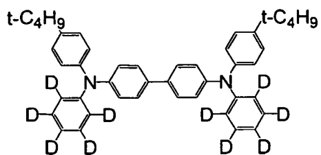
[Chemical Formula 25]
