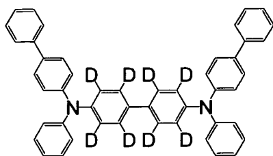
[Chemical Formula 20]
