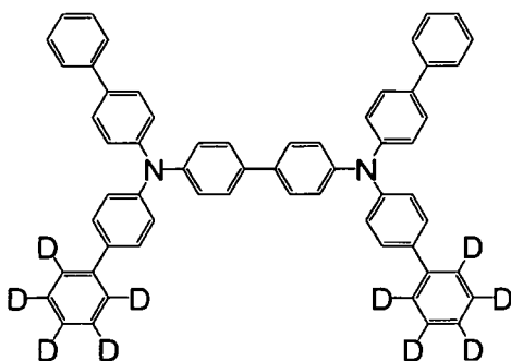
[Chemical Formula 33]
