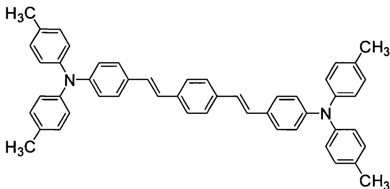
[Chemical Formula 68]
