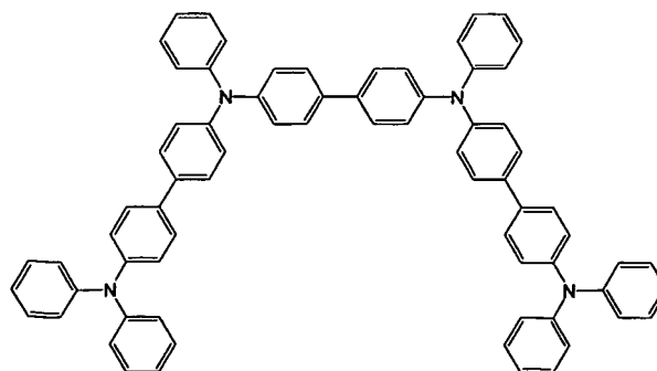
[Chemical Formula 67]
