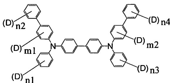
[Chemical Formula 13]
