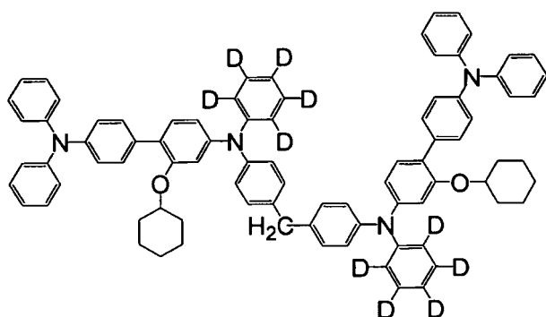
[Chemical Formula 61]
