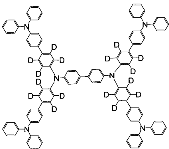
[Chemical Formula 55]
