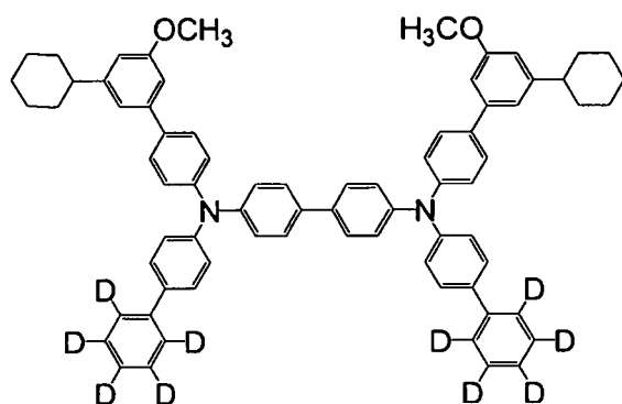
[Chemical Formula 40]
