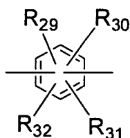
[Chemical Formula 2]
