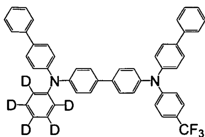
[Chemical Formula 18]
