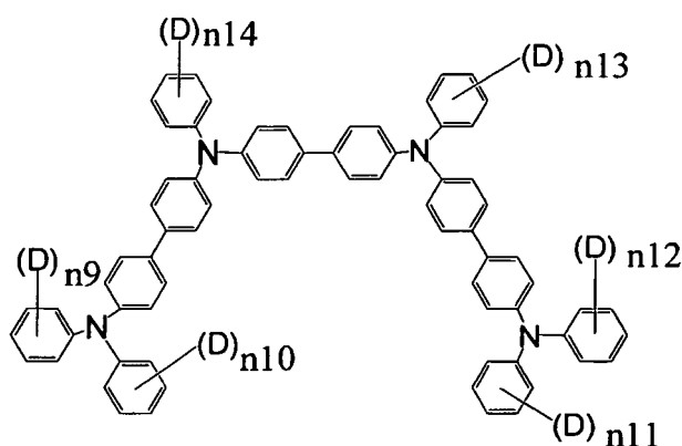
[Chemical Formula 15]
