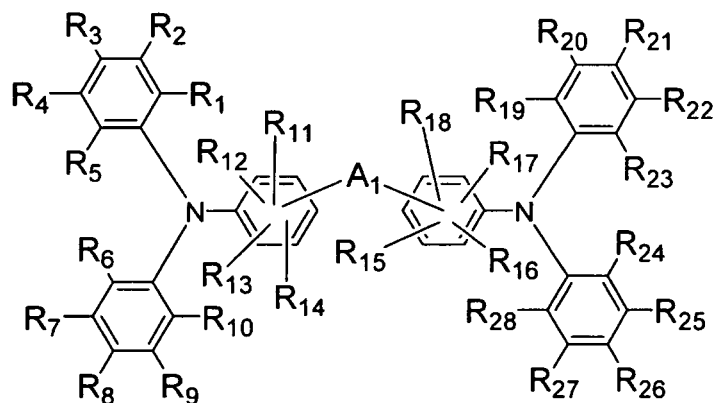
[Chemical Formula 1]
