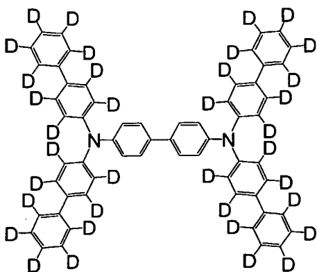
[Chemical Formula 36]
