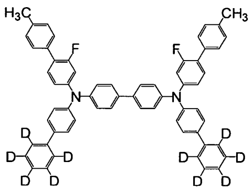
[Chemical Formula 38]
