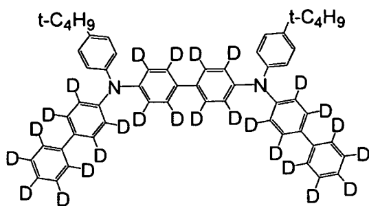
[Chemical Formula 31]
