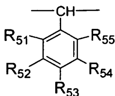
[Chemical Formula 12]
