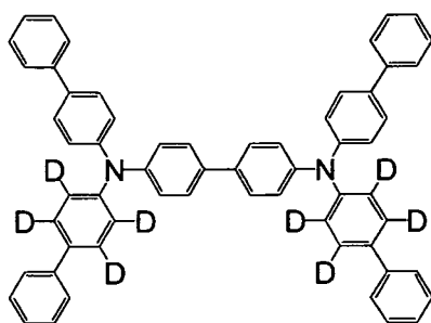
[Chemical Formula 32]
