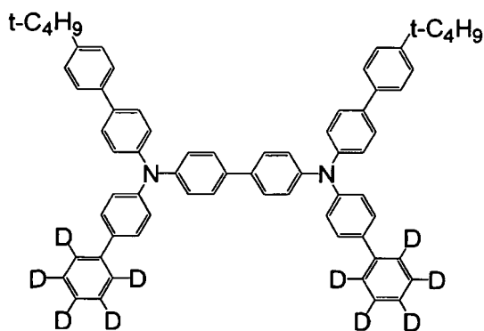
(Compound 25)
