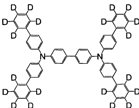
[Chemical Formula 34]
