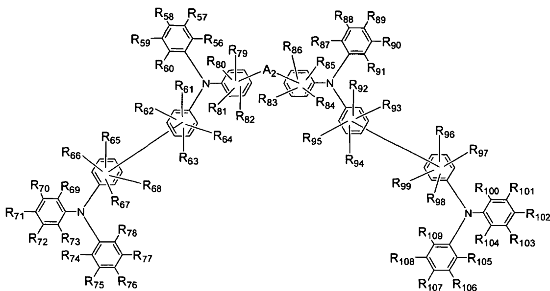
[Chemical Formula 7]
