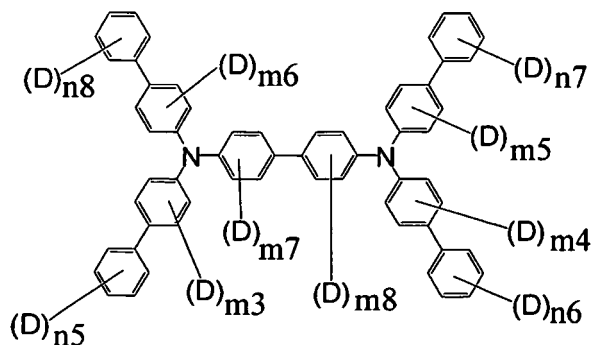
[Chemical Formula 14]
