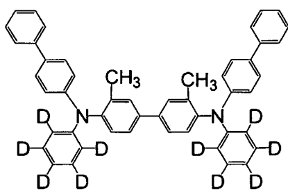
[Chemical Formula 24]
