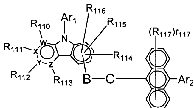
[Chemical Formula 16]
