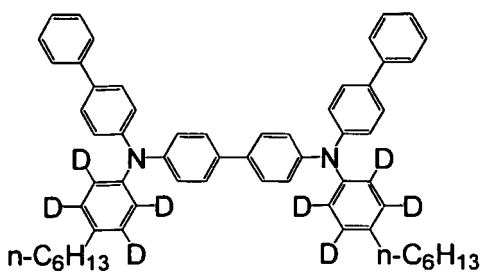
[Chemical Formula 48]
