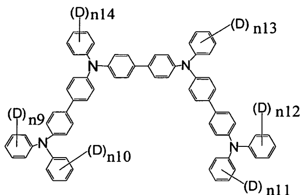
[Chemical Formula 15]
