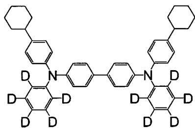
[Chemical Formula 49]
