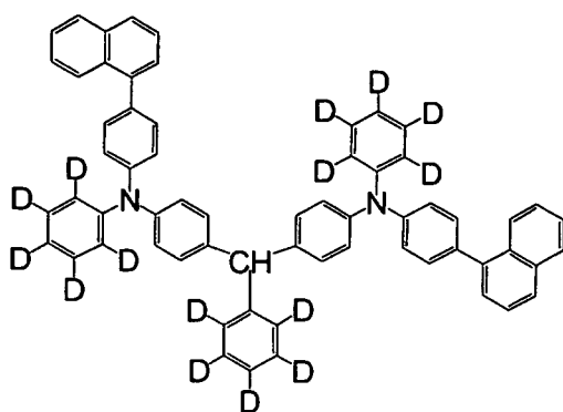
[Chemical Formula 45]
