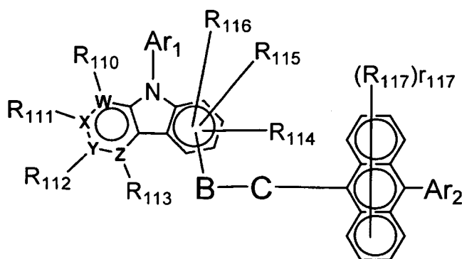
[Chemical Formula 16]
