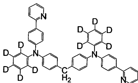
[Chemical Formula 44]
