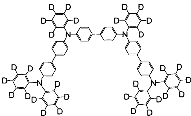
[Chemical Formula 56]
