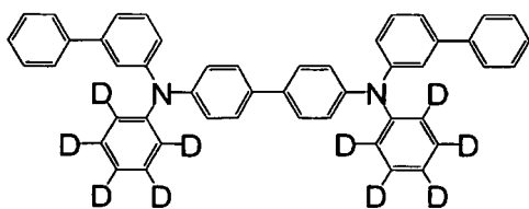
[Chemical Formula 47]
