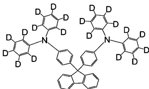
[Chemical Formula 46]
