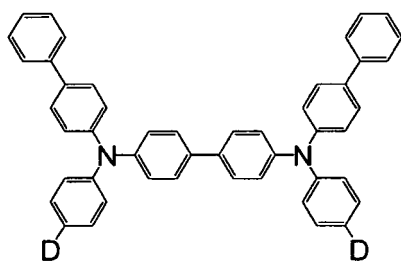
[Chemical Formula 17]
