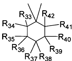
[Chemical Formula 3]
