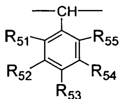
[Chemical Formula 12]
