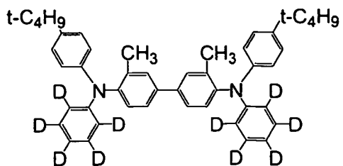
[Chemical Formula 28]
