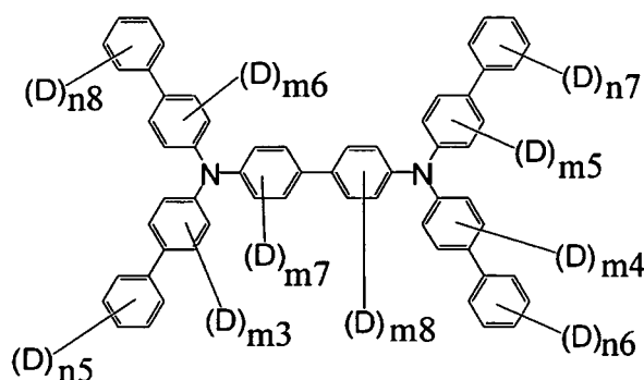
[Chemical Formula 14]
