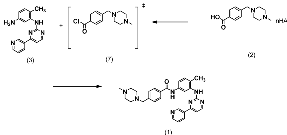
[Reaction Scheme 2]
