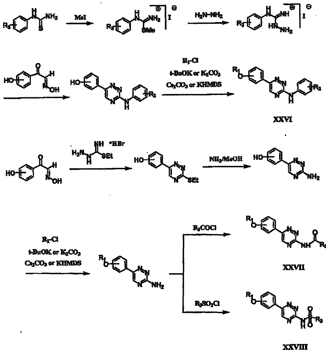
Scheme XVIII
