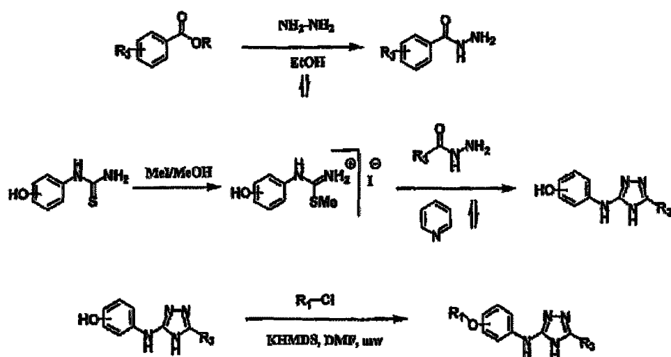
Scheme VIII
