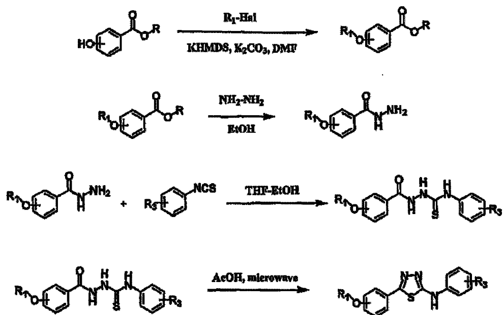
Scheme XV
