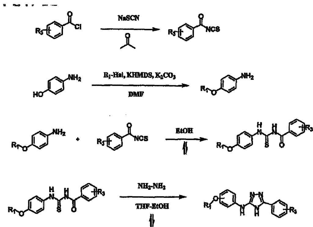
Scheme IX
