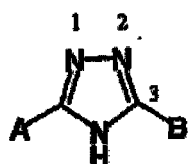
4H-1,2,4-triazole
