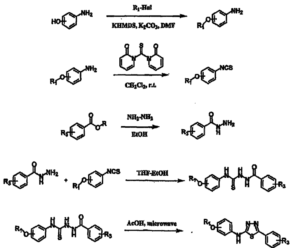
Scheme XVI
