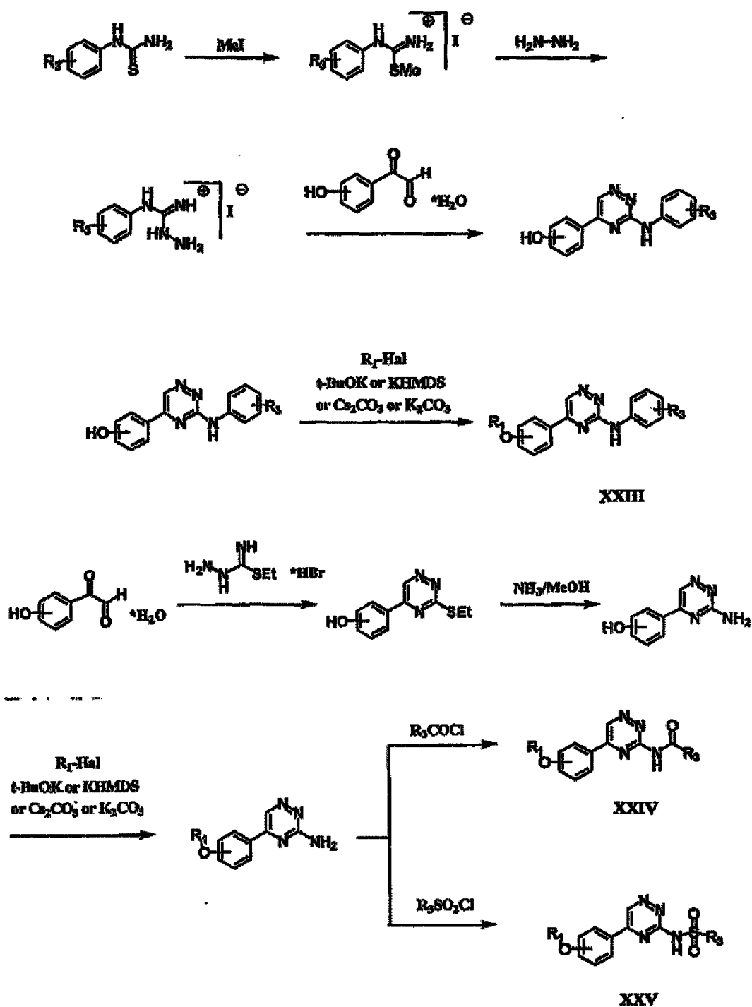
Scheme XVII
