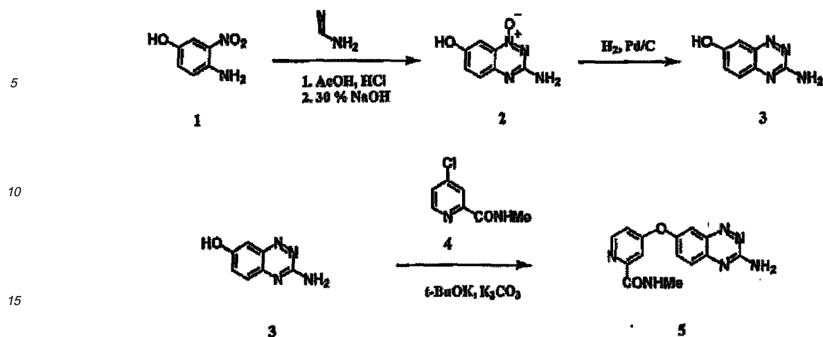
Scheme II
