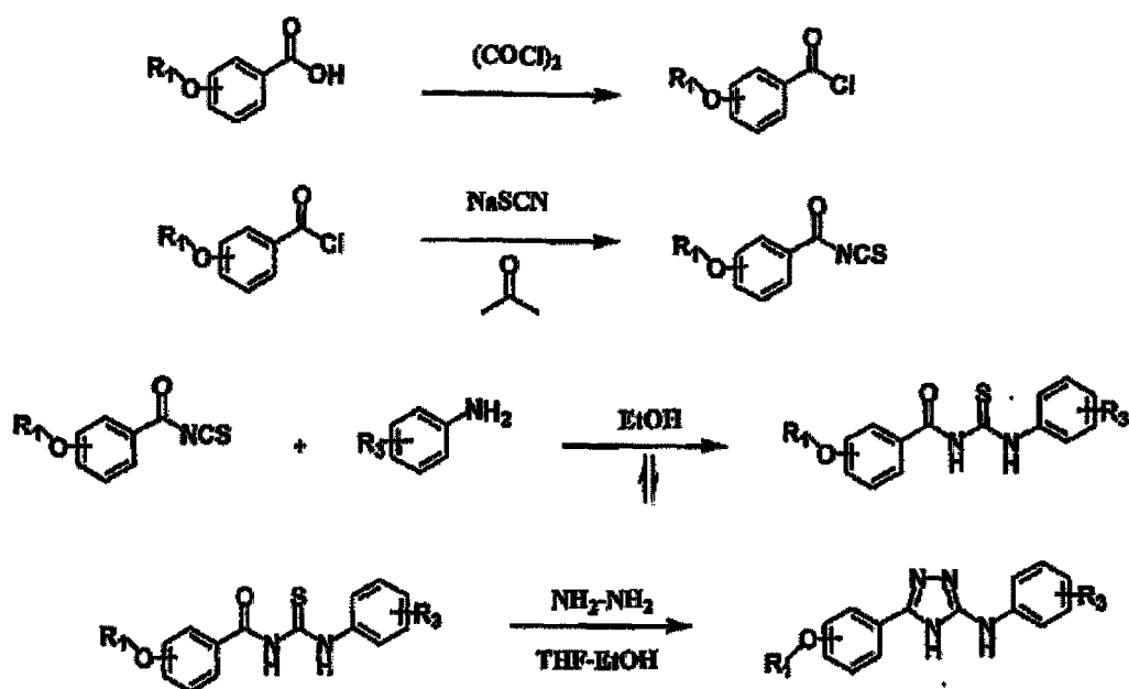
Scheme VII
