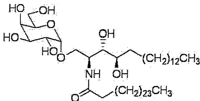
Compound 1 (RN7000)
