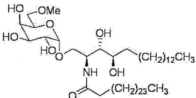
Compound 4 (RCAI-61)
