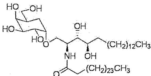
Compound 3 (RCAI-56)
