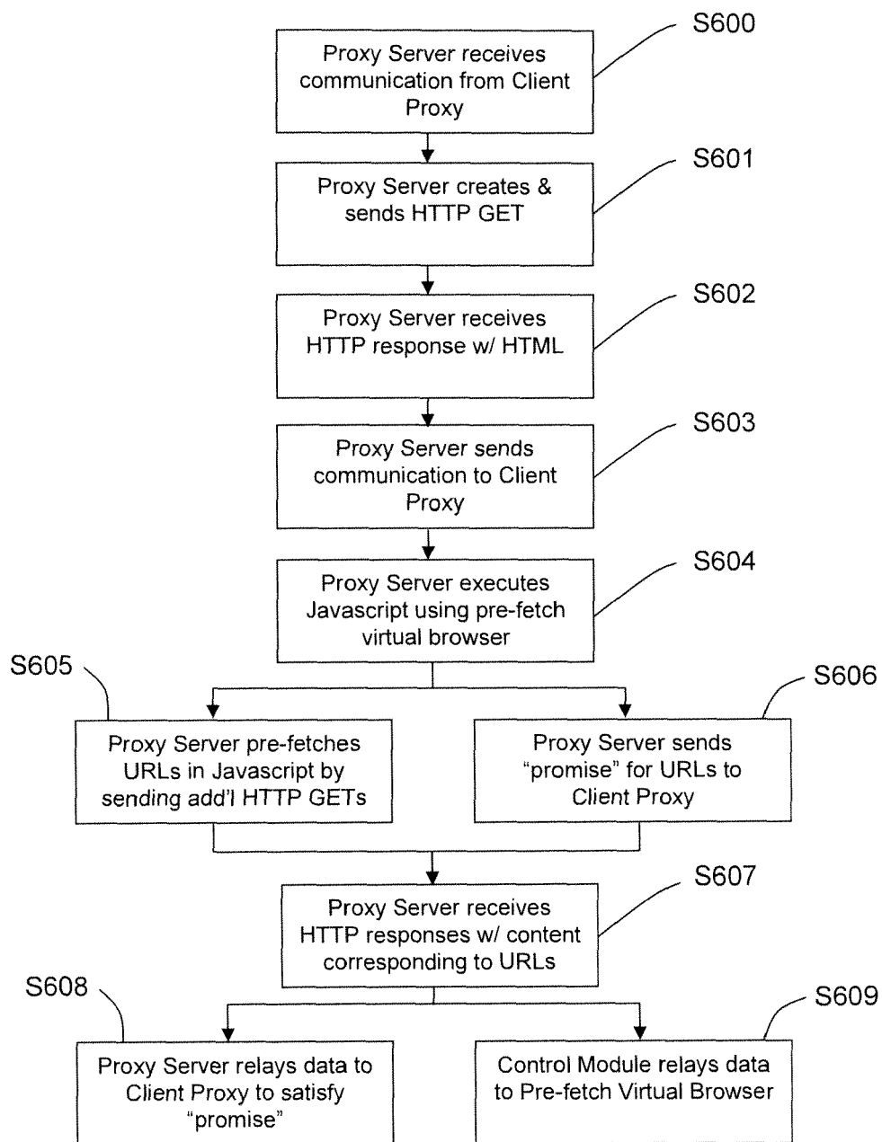
Fig. 6 Proxy Server Pre-Fetching
