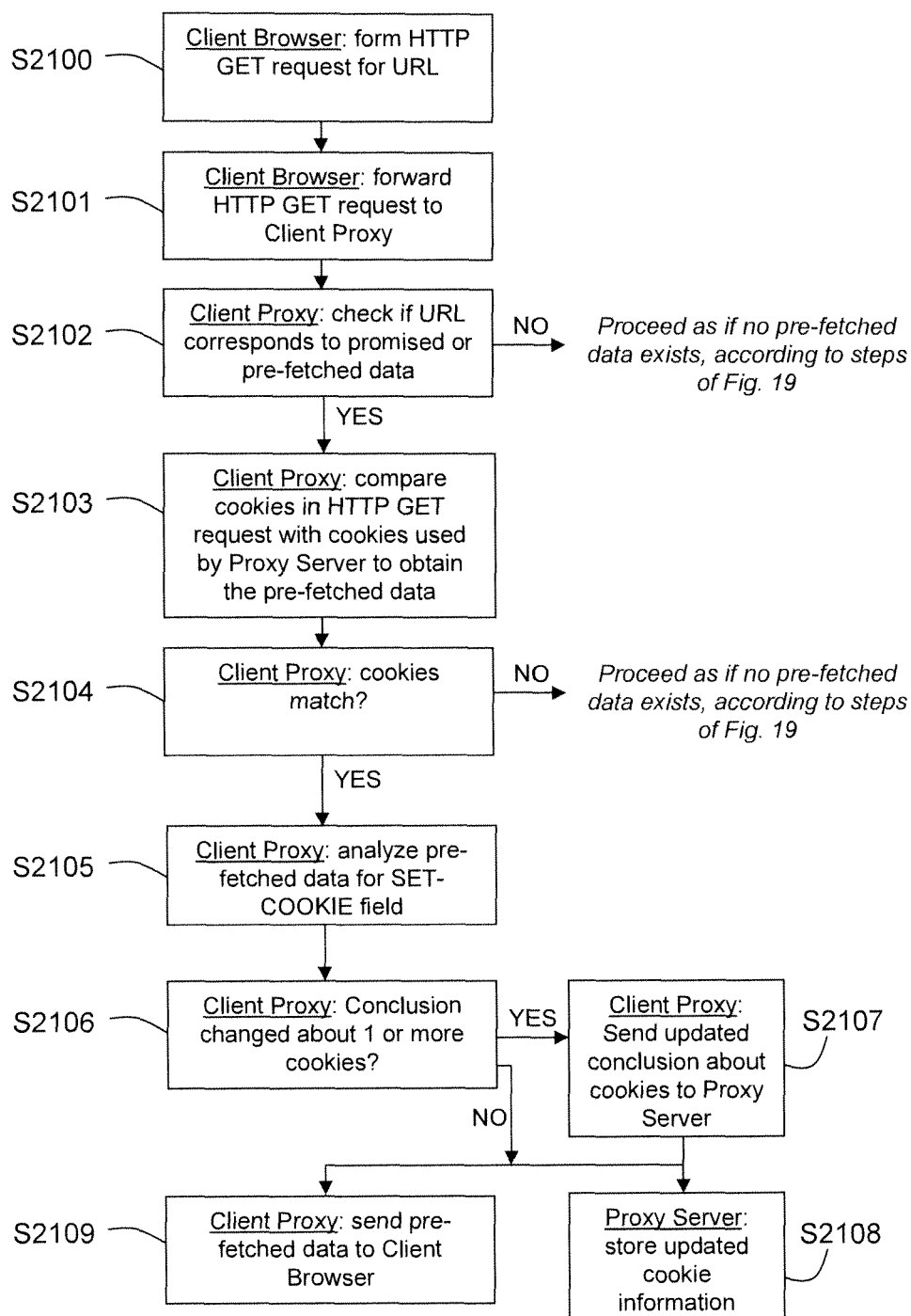
Fig. 21 Cookies tracking (When Client Proxy contains promised/pre-fetched data)
