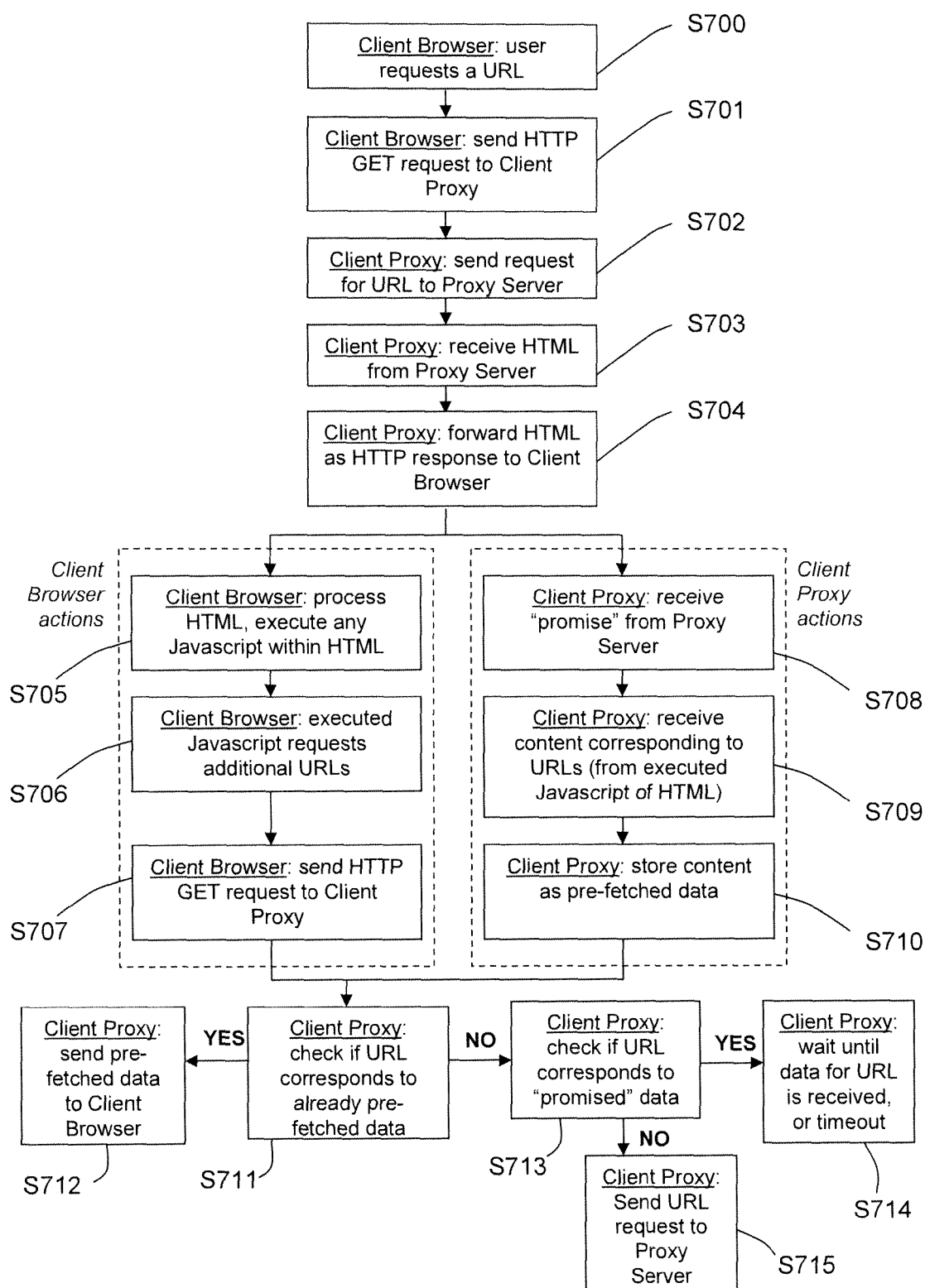
Fig. 7 Client/Client Proxy Pre-Fetching
