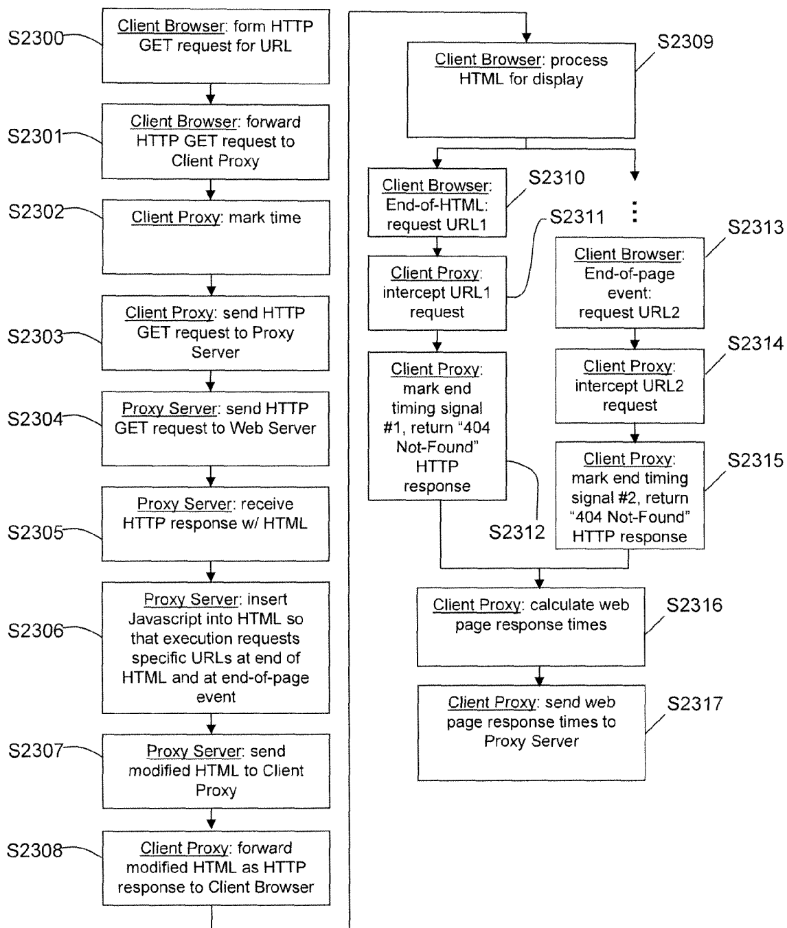
Fig. 23 Web Page Response Time
