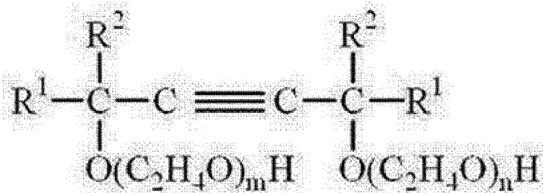
Formula (1)
