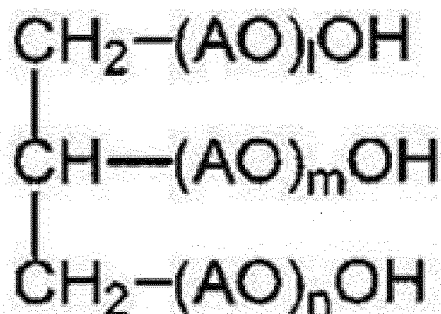
Structural Formula (1)
