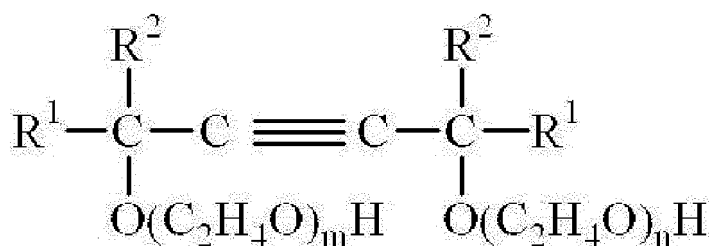
Formula (1)
